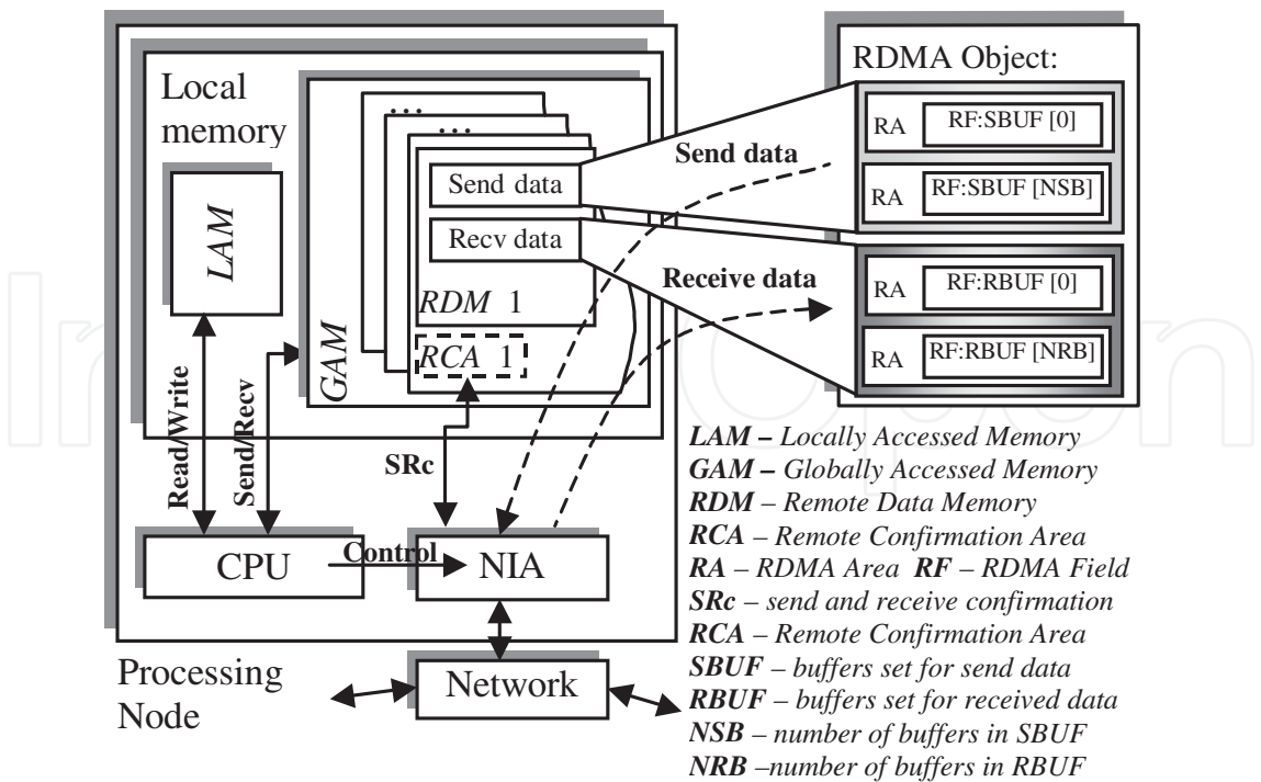
Fig. 7. Memory Structure in Rotating-Buffers Method (For One processing Node on the HITACHI SR2201 supercomputer).
