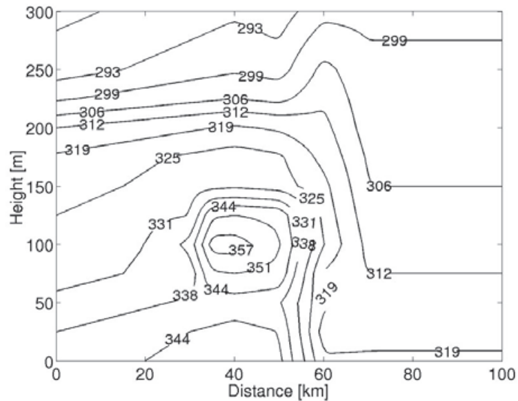
Fig. 4. 2D panel of the atmosphere charachteristics. Contour lines report the value of the refractivity index N
