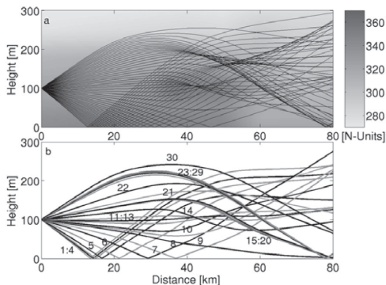
Fig. 6. Ray pattern (top) and wavefronts (bottom)
