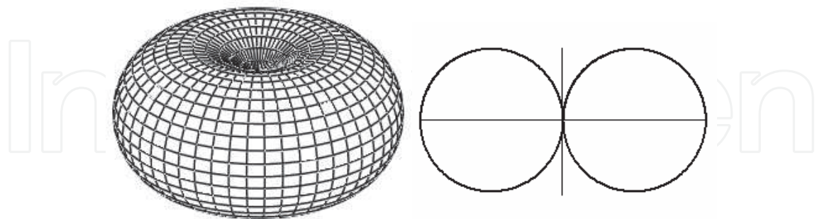
Fig. 3. Directivity diagram of the Hertzian dipole, the isotropic medium ( \epsilon = \epsilon_1 = 1 ) which is a constant at various values of radius of sphere, where \bar{H} is complex conjugate function.
