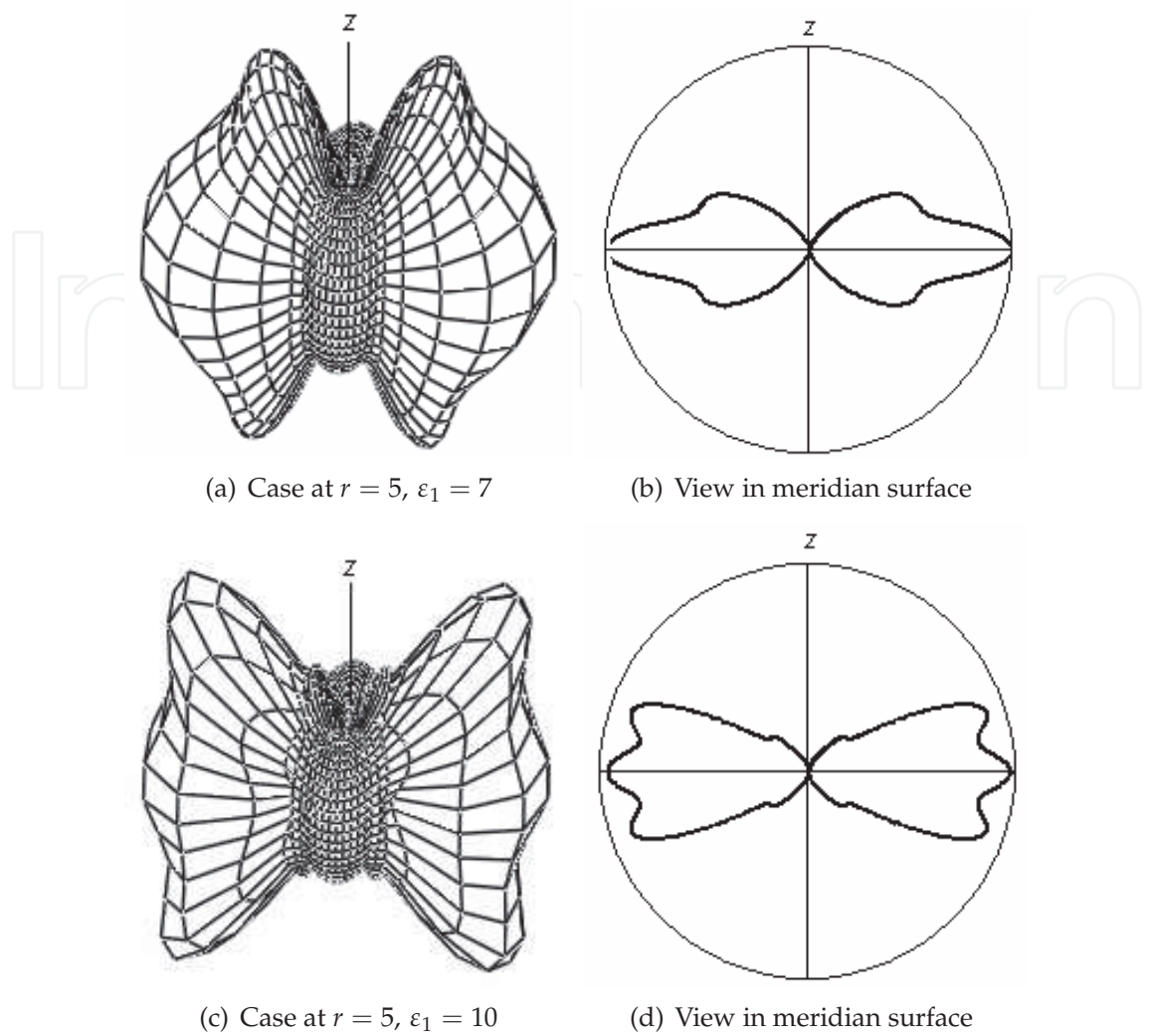
Fig. 2. Directivity diagram, the axis of dipole ( z ) is perpendicular to axis of a crystal
