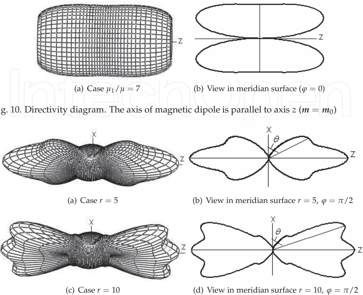
Fig. 11. Directivity diagram. The axis of magnetic dipole is perpendicular to z, \mu_1/\mu = 7
