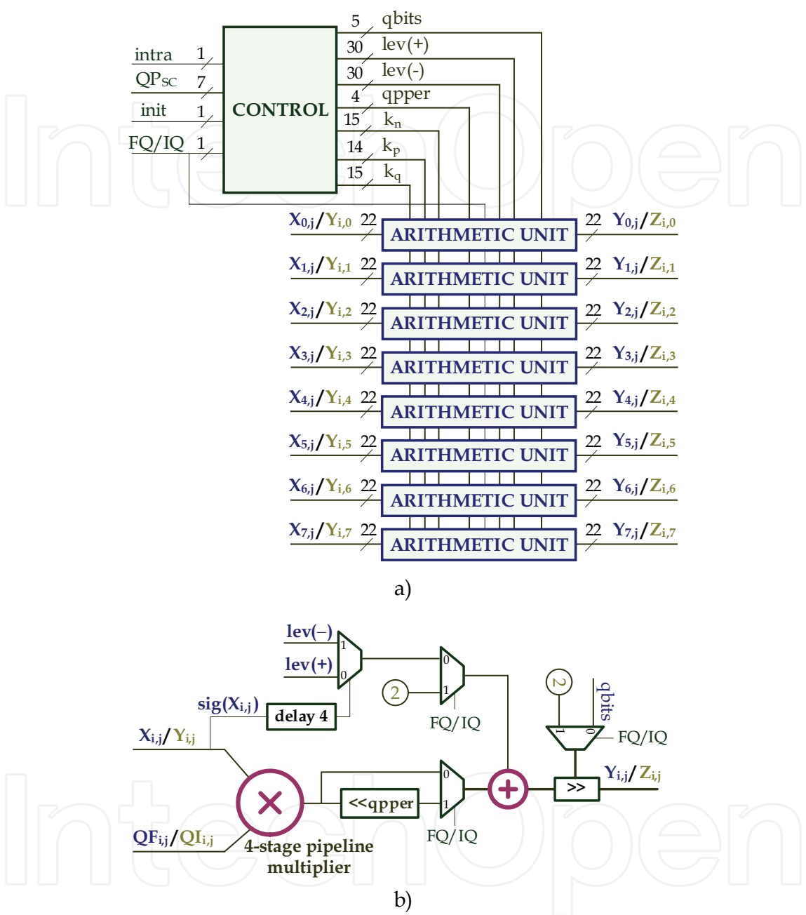
Fig. 6. Configurable forward quantizer and scaling module: a) Block diagram, and b) Schematic of the arithmetic unit.
