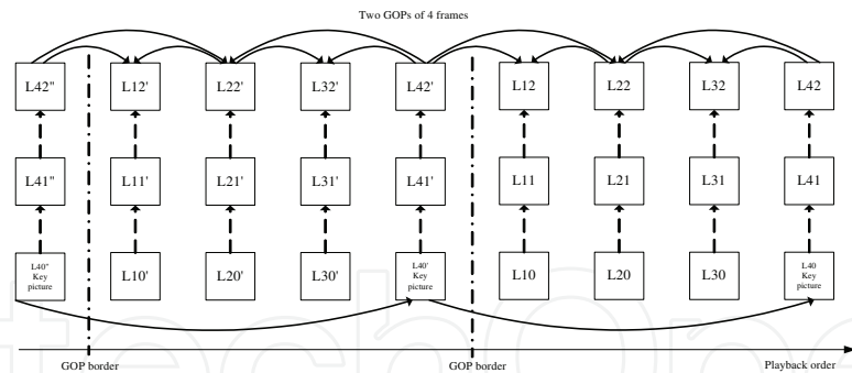
Fig. 1. GOP structure of SVC.
