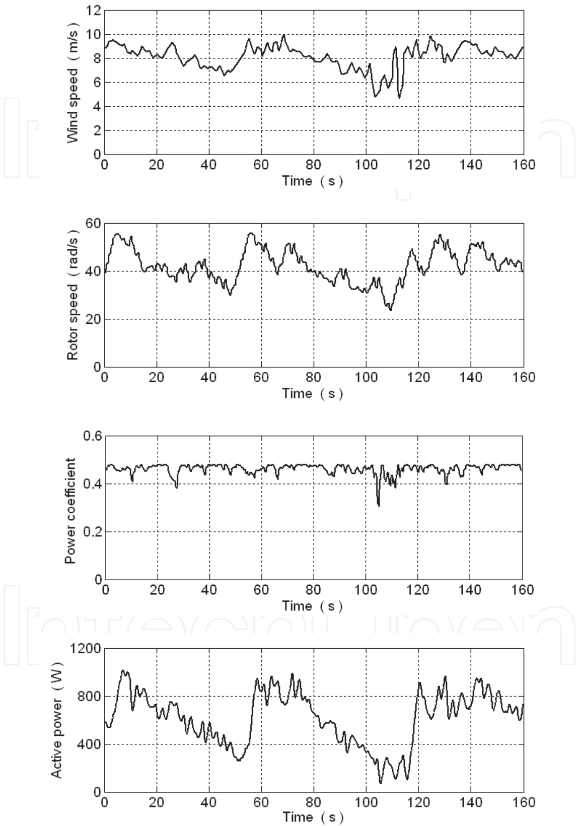
Fig. 21. Operation of the WECS under real wind speed profile.
