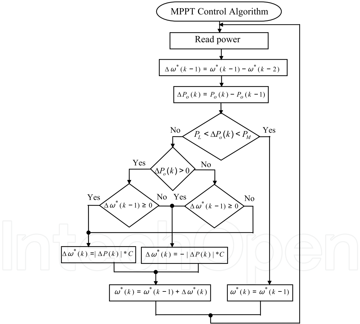
Fig. 19. Flow chart of MPPT controller.
