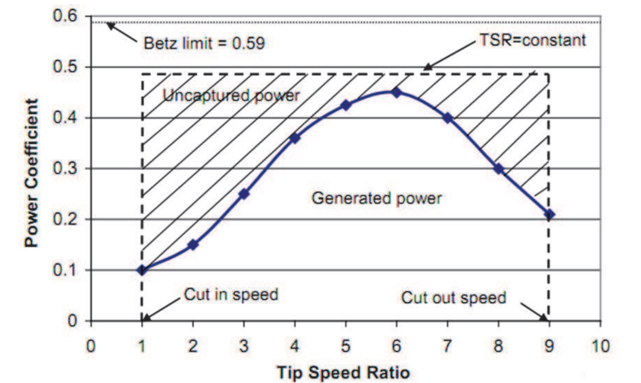
Fig. 4. Power coefficient as a function of TSR for a two-bladed rotor.
