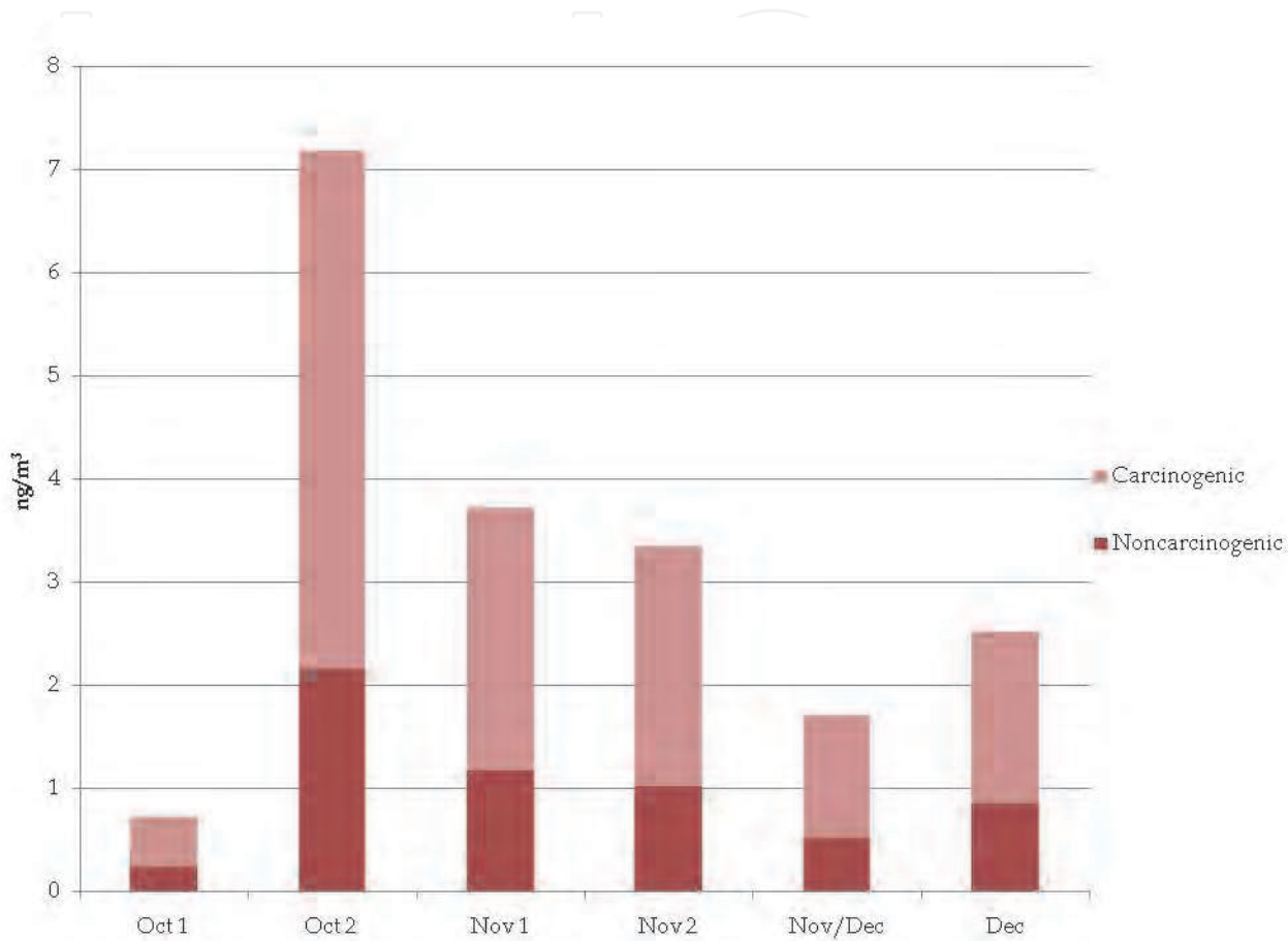
Fig. 6. Concentrations of potentially carcinogenic PAHs (ng/m³) according to IARC (2010) in PM10 samples from an urban area under the influence of oil refinery plant.
