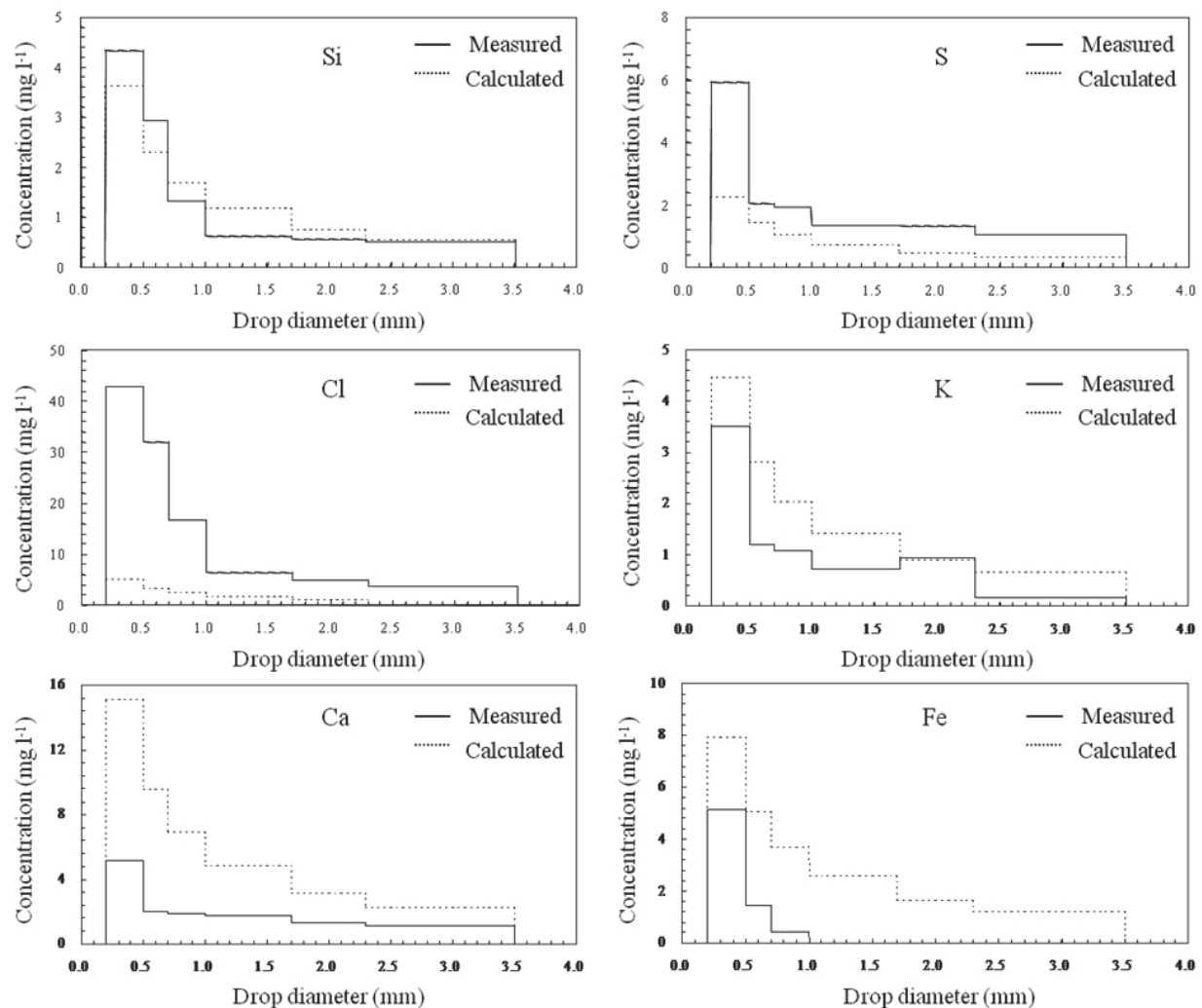
Fig. 13. The plotting of calculated vs. measured mass concentrations for six major elements as a function of raindrop size
