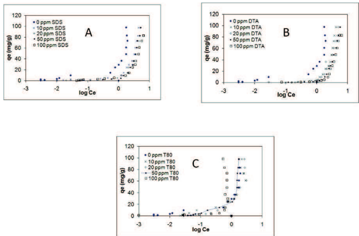
Fig. 16. Zimm-Bragg isotherms for ALG-DB22 (CaCl 2 ) with different amounts of surfactant A) SDS, B) DTA C) T 80.
