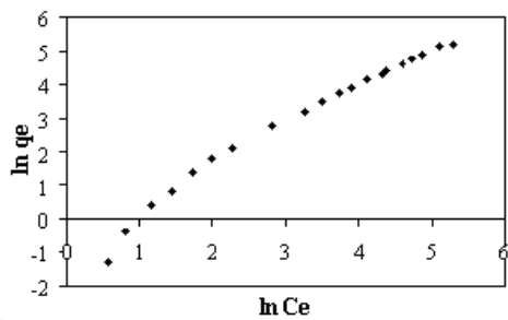
Fig. 8. Plot of \ln q_e versus \ln C_e to obtain Freundlich parameters ( K_F and 1/n parameters) in system ALG-DY54 (HCl). (with permission of J. Mex. Chem. Soc.) The values of the Freundlich constants together with the correlation coefficient are presented in table 2.
