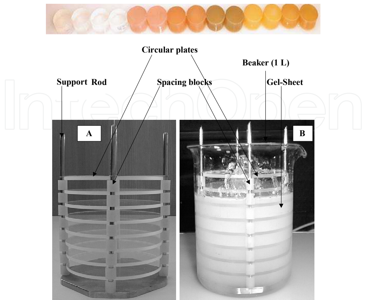
Fig. 7. Parallel plates equipment for making uniform k-carrageenan gel disks.
