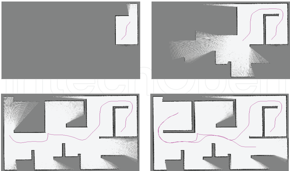
Fig. 12. Simulation results with method 2, without final objective. Trajectory calculated.
