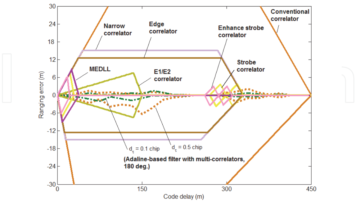
Fig. 11. Code-phase error simulation results of existing methods. ( \alpha_0 = 1.0 , \alpha_1 = 0.5 , \tau_0 = 0 chip, \tau_1 = 0 \sim 1.5 chip, \theta_0 = 0^\circ , (\theta_1 = 0^\circ, 180^\circ) ).
