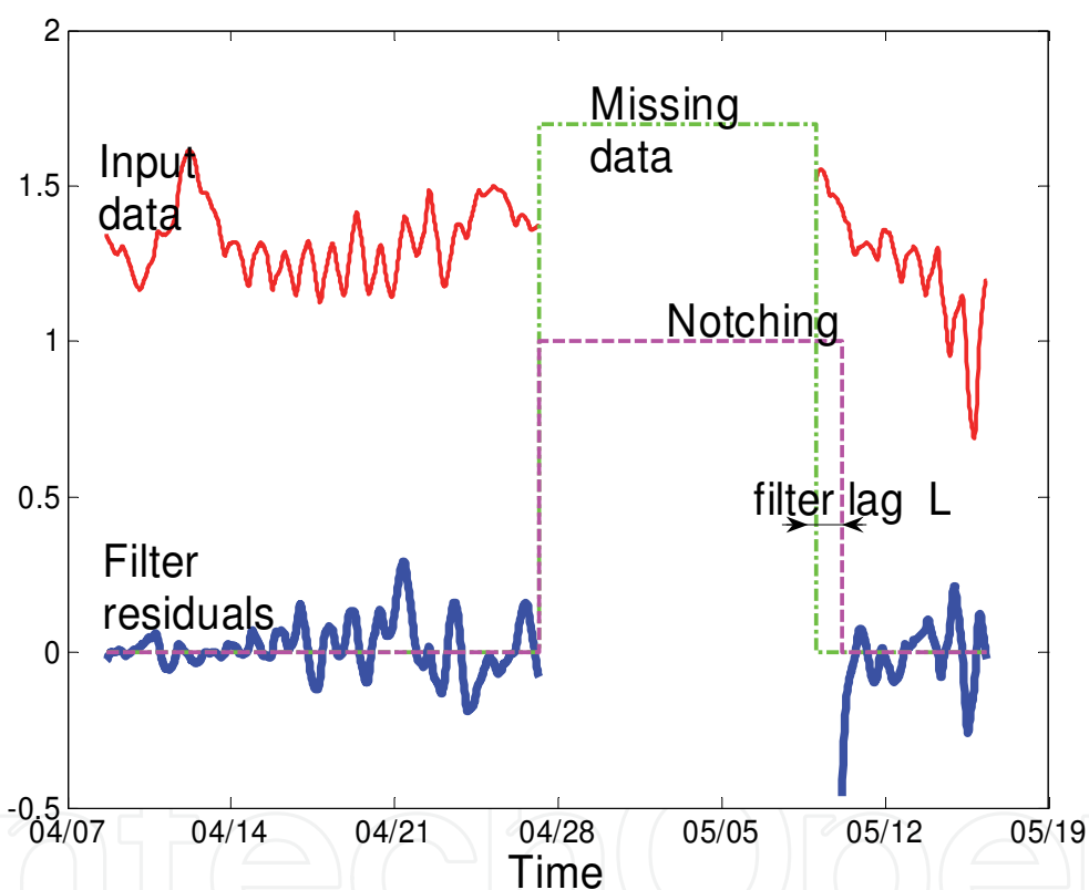
Fig. 15. Time notching in adaptive filtering.
