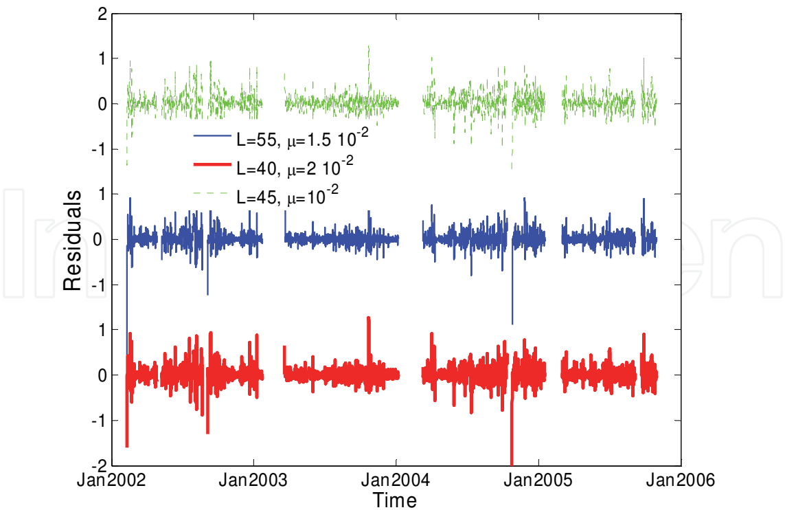
Fig. 16. Residuals of the adaptive filters applied on y_{MA}(t) data using three different combinations of the learning rate and the filter length.
