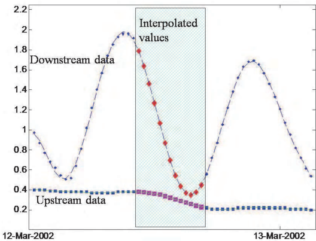
Fig. 8. The treatment of the missing values.
