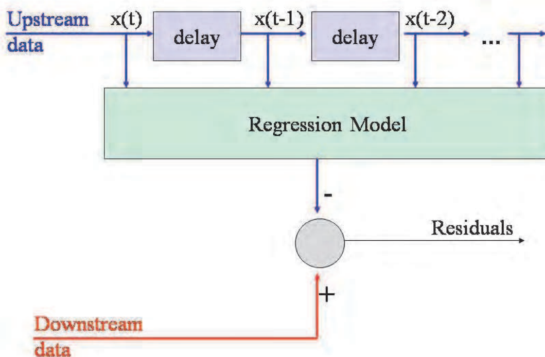
Fig. 14. Removal of the upstream data influence.
