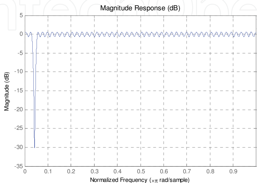
Fig. 10. Magnitude response of the first filter.
