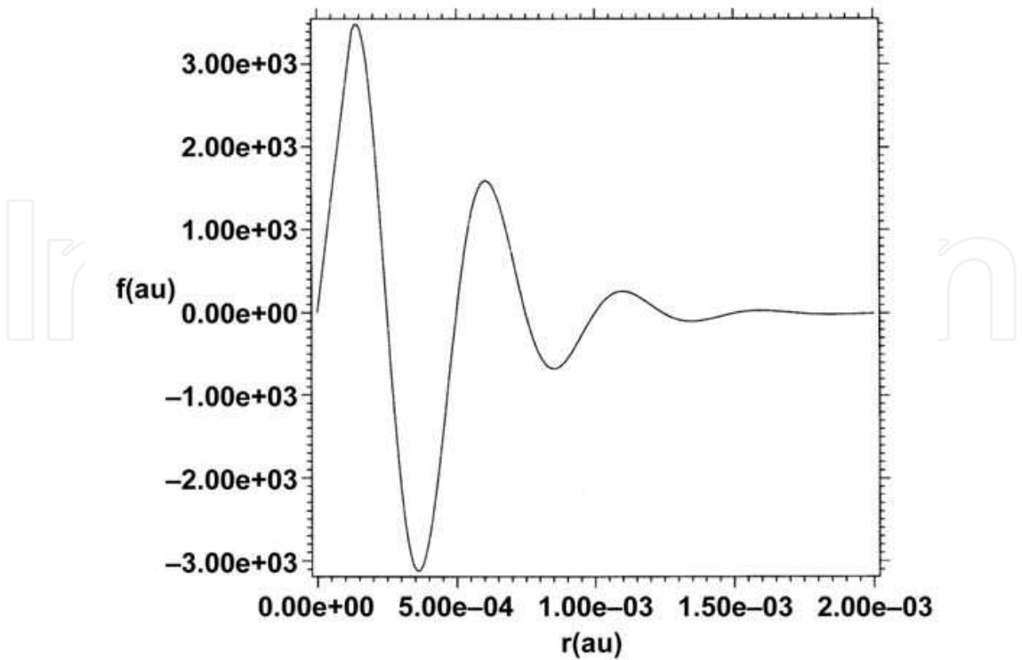
Fig. 5. Simulation using Eqs. (22)-(23) of the wave function shown in Fig. 4. The simulated wave function is unnormalized.
