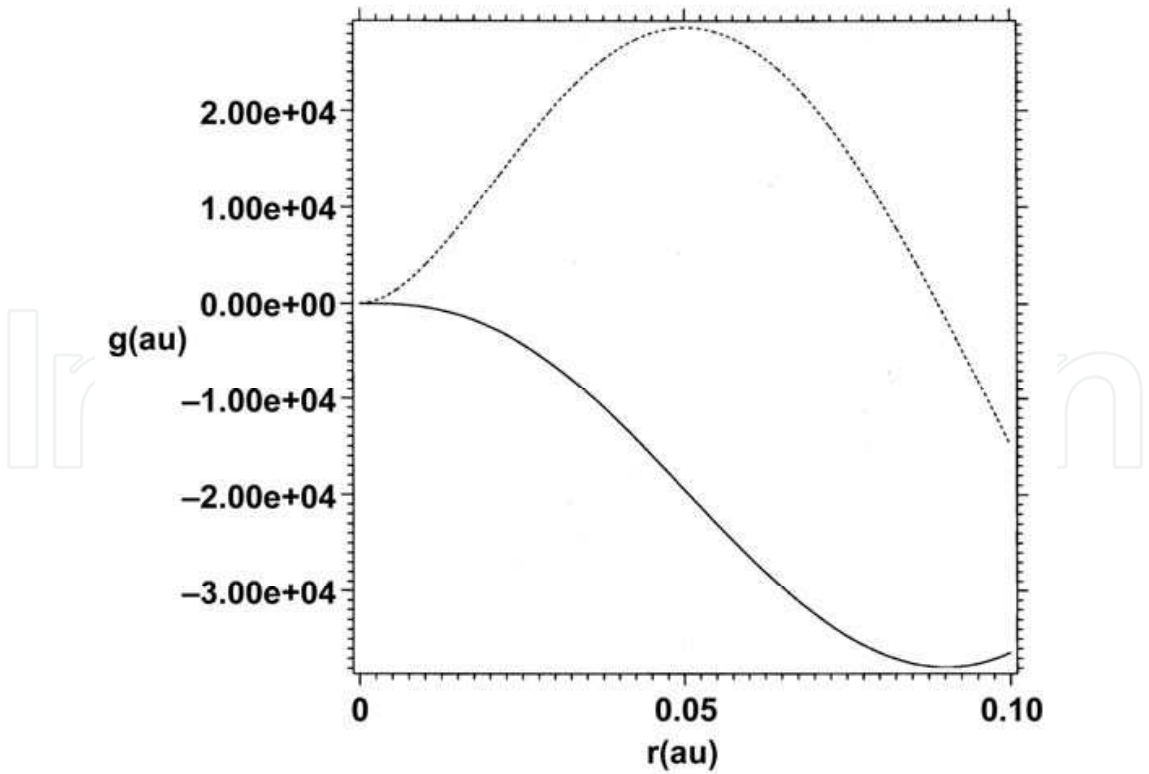
Fig. 6. Unnormalized wave function obtained from Eq. (23) by outward integration. Solid: real part. Dashed: imaginary part.
