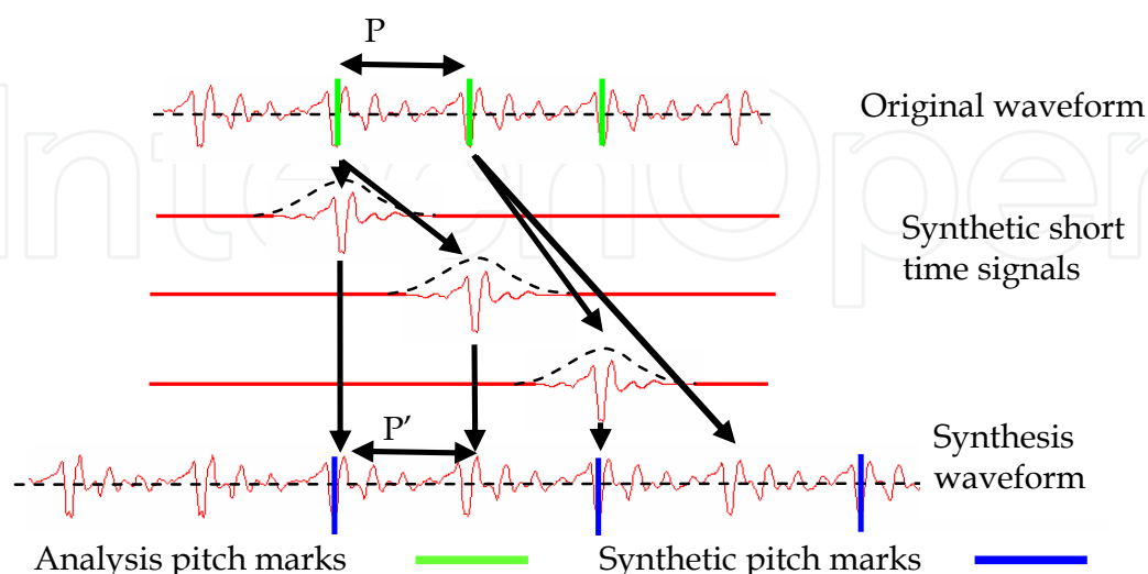
Fig. 1. Example of slowing down: the duration of the original signal is lengthened by a factor 2 ( P' = 2P ).
