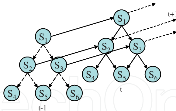
Fig. 15. An example of Dynamic Bayesian Networks (DBNs)
