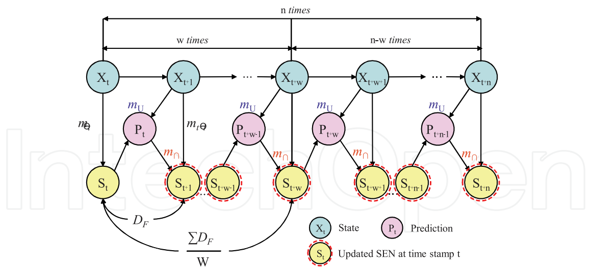
Fig. 6. The Proposed DEN for n time intervals
