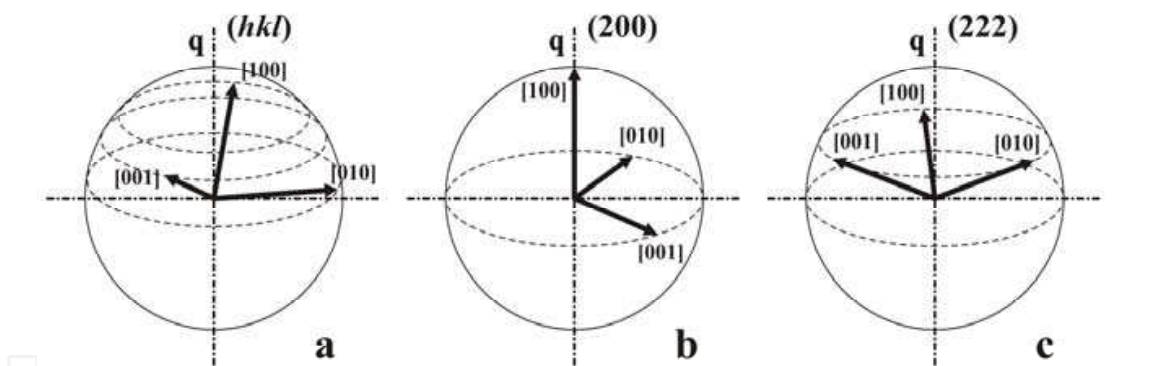
Fig. 10. Orientations of the axes of the nanocrystals contributing to the (hkl) reflection in the X-ray diffraction pattern measured during (a) the \theta - 2\theta scanning along the scattering vector q and (b, c) special cases for the (b) (200) and (c) (222) reflections.
