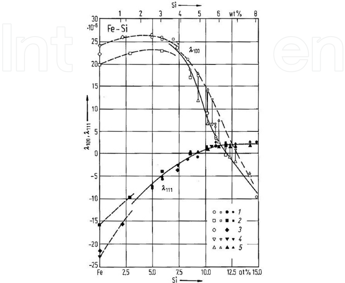
Fig. 15. Magnetostriction constants as functions of Si concentrations, determined by strain-gauge measurements on single crystals (room temperature). Large symbols: slowly cooled specimens. Small symbols: specimens quenched from temperature of the order of 1000°C. Image was taken from the database (Bertotti & Fiorillo, 1994c), Fig. 42.
