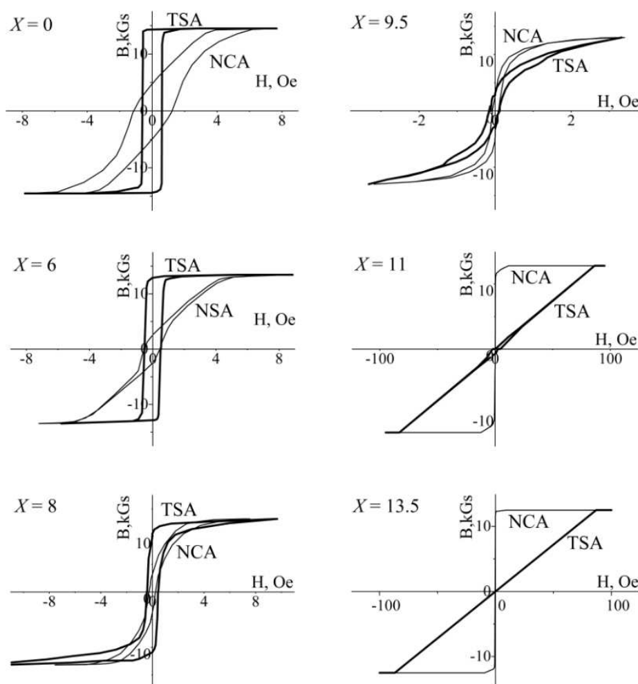
Fig. 1. Hysteresis loops measured for nanocrystalline \text{Fe}_{87-X}\text{Si}_X\text{B}_9\text{Nb}_3\text{Cu}_1 alloy after the nanocrystallization annealing (NCA) and tensile stress annealing (TSA).
