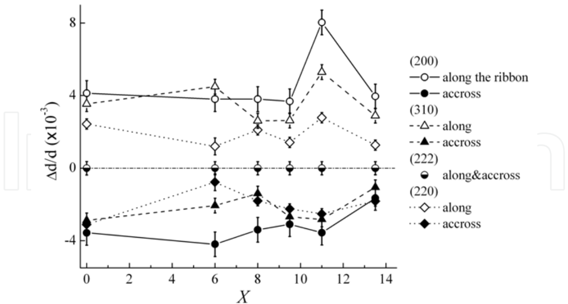
Fig. 9. Dependence of relative extension (along the ribbon) and compression (across the ribbon) of the nanocrystal lattice for the interplanar spacings (200), (220), (310) and (222) on the silicon content X .
