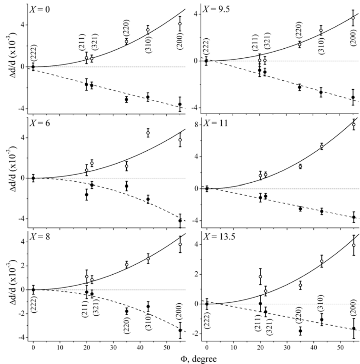
Fig. 8. Relative changes in the interplanar spacing \Delta d/d : longitudinal strains ( \circ ), and transverse reductions ( \bullet ) in the alloys with different silicon content X depending on the angle \Phi between the direction [hkl] and the closest axis \langle 111 \rangle . Lines show the variants of fitting by linear or quadratic functions of the angle. The distortions of the nanocrystal structure in the \text{Fe}_{87-X}\text{Si}_X\text{B}_9\text{Nb}_3\text{Cu}_1 alloy sample subjected to the TSA treatment observed experimentally can be interpreted as follows. In the case of measurements in the transmission geometry, the sample is adjusted so that, during \theta - 2\theta scanning, the scattering vector \mathbf{q} is always in the sample plane. In this case, all the nanocrystals, for which the normals to the (hkl) planes are parallel to the scattering vector \mathbf{q}_{hkl} within the limits of the instrumental resolution, will contribute to the (hkl) reflection in the X-ray diffraction pattern and the position of the maximum in \theta angles \theta_{hkl} will indicate the mean distance between the (hkl) planes in the direction of scanning.
