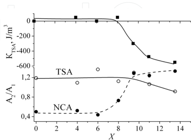
Fig. 13. Variation of the anisotropy constant K_{TSA} and of the ratio A_2/A_1 as functions of the silicon content X for the alloys subjected to NCA (•) and TSA (○).
