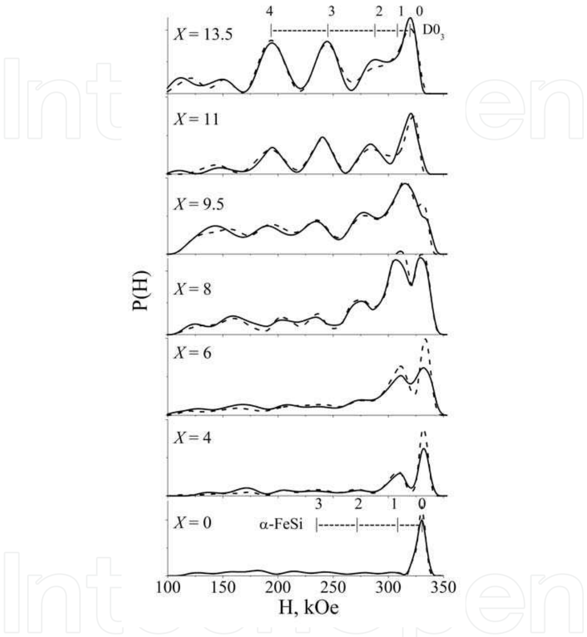
Fig. 12. P(H) , distribution functions of HFFs of the nanocrystalline alloys Fe_{87-X}Si_XB_9Nb_3Cu_1 with different values of X after NCA (dashed curves) and TSA (solid). With the rulers marked \alpha -FeSi and D0_3 the line positions are shown corresponding to surroundings with 0, 1, 2, and 3 silicon atoms in the first coordination sphere for the disordered state and to surroundings with 0, 1, 2, 3 and 4 silicon atoms for the ordered state, respectively.
