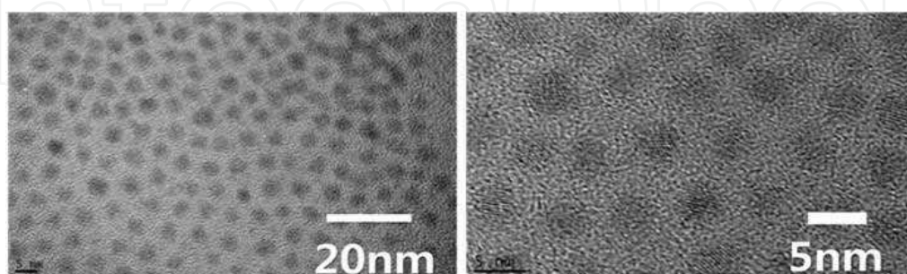
Fig. 3.2. TEM image of CdSeS nanocrystal grown for 2 minutes at 300^\circ\text{C} under \text{N}_2 flow with [\text{Cd}]/([\text{Se}]+[\text{S}]) \gg 1 .
