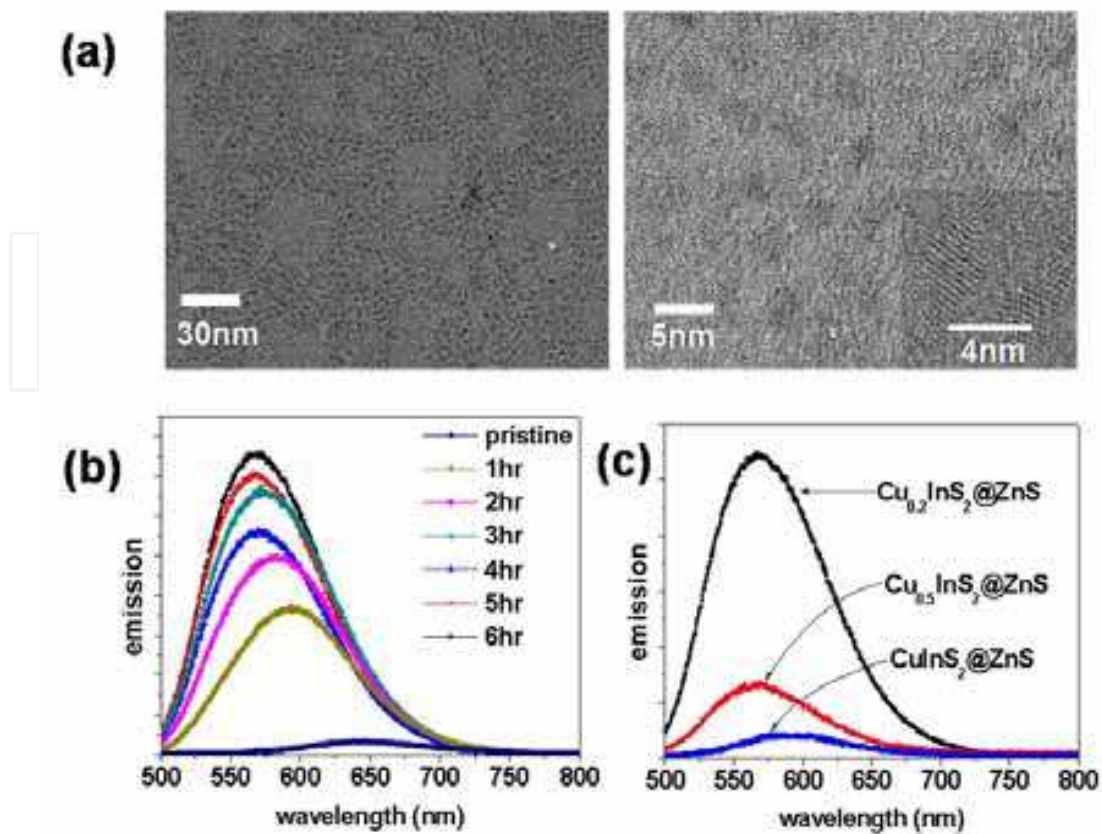
Fig. 3.10. (a) TEM images of \text{Cu}_{1-x}\text{InS}_2 nanocrystals ( x=0.8 ) treated with zinc acetate and palmitic acid for 5 hours at 230°C. (b) Temporal evolution of PL of \text{Cu}_{1-x}\text{InS}_2 nanocrystals ( x=0.2 ) (c) PL of \text{Cu}_{1-x}\text{InS}_2 NCs with various starting composition ( x=0, 0.5, 0.8 ) after refluxing with zinc acetate and palmitic acid for 5 hours at 230°C.
