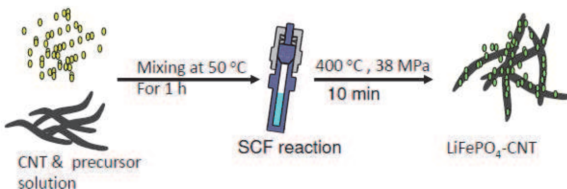
Fig. 10. Schematic illustration of preparation of the LiFePO 4 decorated MCNT by using SCE process.
