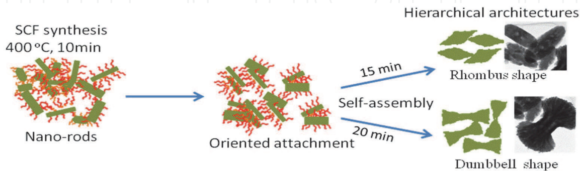
Fig. 7. Schematic illustrations of formation mechannism and growth of the \text{LiFePO}_4 nanorods and rhombus and dumbbell shape hierarchical nanostructure by nano rods self assembly.
