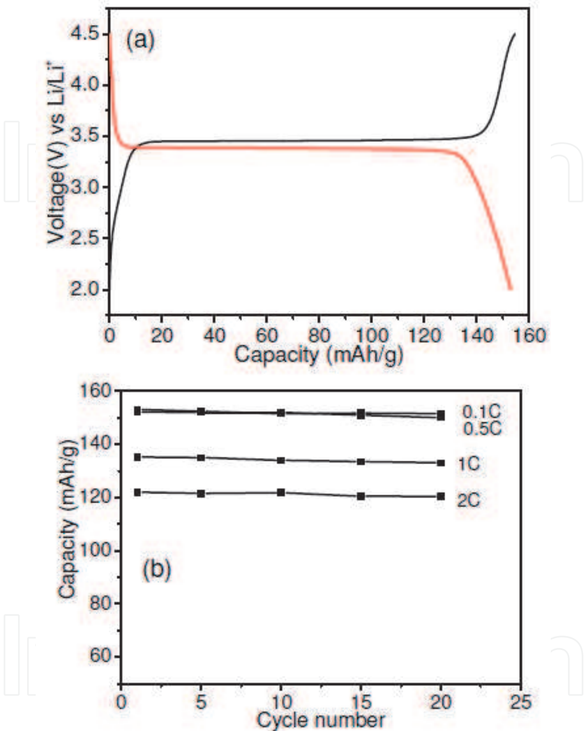
Fig. 9. Charge-discharge profile of the LiFePO 4 hierarchical nanostructure measured at 0.1 C (a), along with the rate capability and cyclic performance (b).
