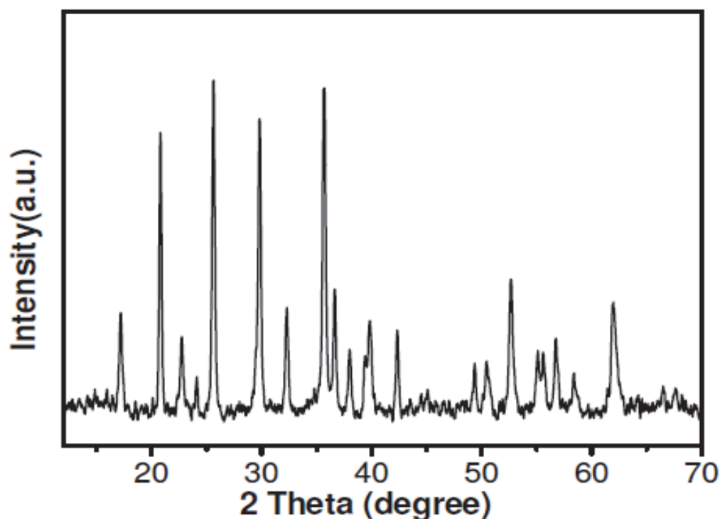
Fig. 11. XRD pattern of the LiFePO 4 decorated MCNT nano composite synthesized under SCE conditions at 400 °C for 10 min reaction.
