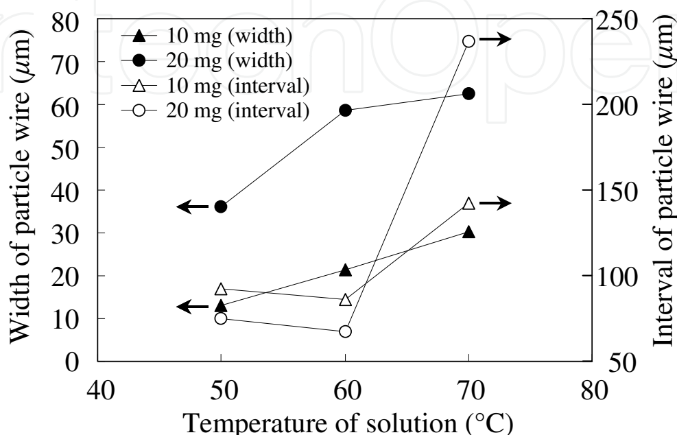
Fig. 17. Width and interval of particle wires as functions of temperature of solution.
