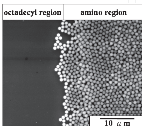
Fig. 8. SEM micrograph of randomly deposited \text{SiO}_2 particles in the amino region. Reprinted with permission from Ref. 23 , Masuda, Y., Itoh, M., Yonezawa, T. and Koumoto, K., 2002, Langmuir , 18, 4155. Copyright @ American Chemical Society
