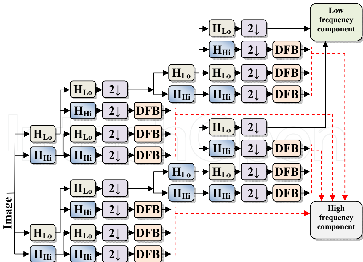
Fig. 3. The proposed of DT-CCT based on Fusion Rules.
