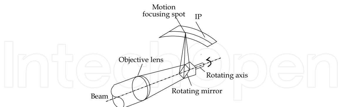
Fig. 5. Scanning with a single mirror
