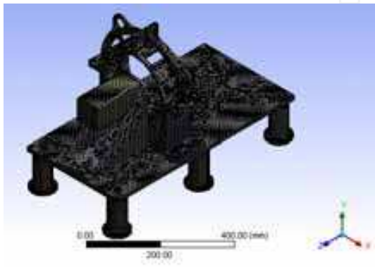
Fig. 31. Finite element mesh of the structure
