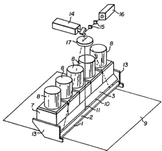
Fig. 7. Optical system of a CR scanner
