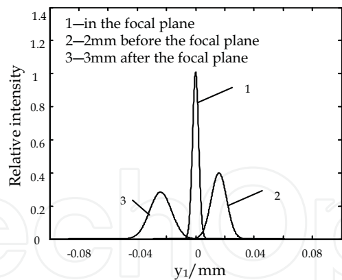
Fig. 28. Intensity distribution of different locations
