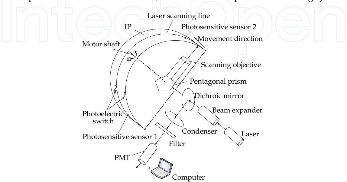
Fig. 9. Structure diagram of the CR scanner
