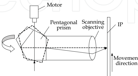
Fig. 24. Pentagonal prism with installation error
