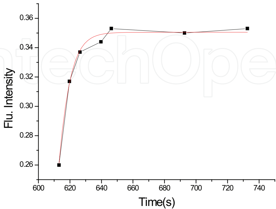
Fig. 5. Recovery profile for pure PE capsule measured by CLSM (black dot is recorded by CLSM, red line is the fitted curve)
