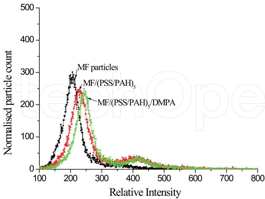
Fig. 6. Normalized light scattering intensity distributions of uncoated MF particles, MF coated with (PSS/PAH) 5 and MF/ (PSS/PAH) 5 /DMPA, respectively. The diameter of MF particles used in experiment is 1.08 ± 0.10 μm.
