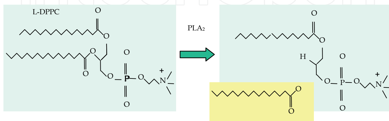
Fig. 10. Scheme for PLA 2 catalyzed L-DPPC reaction
