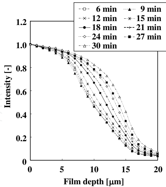
Fig. 26. Relationship between the depth of OCA sample and I_s at several times after addition of perylene/TEGDA mixture.
