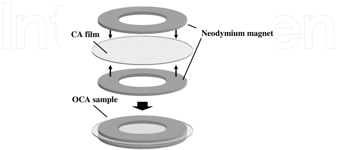
Fig. 22. OCA sample fixed between neodymium magnets.
