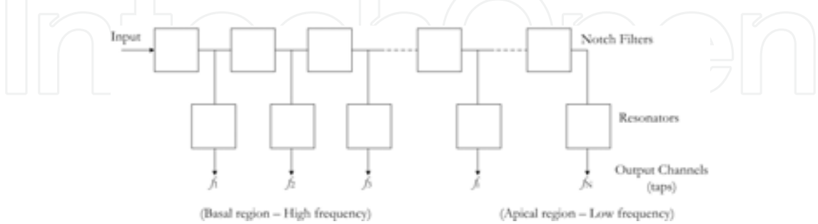
Fig. 1. Block diagram of the cascade/parallel filterbank for modelling travelling wave propagation in the BM; adapted from Lyon (Lyon, 1982).
