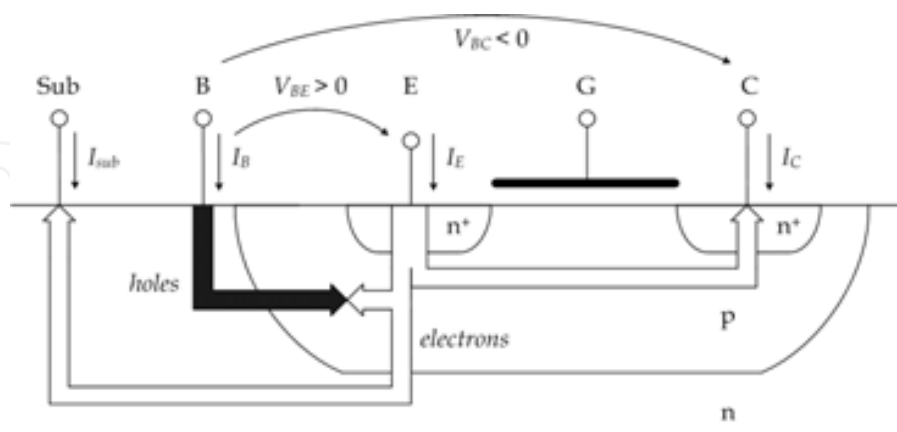
Fig. 20. Bipolar operation of a MOS device; adapted from Van Schaik (A. Van Schaik et al., 1996).
