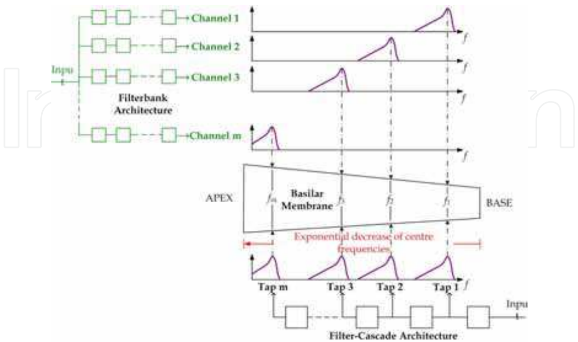
Fig. 12. Modelling BM filtering via neuromorphic (filter-cascade) and bio-inspired (filterbank) architectures.
