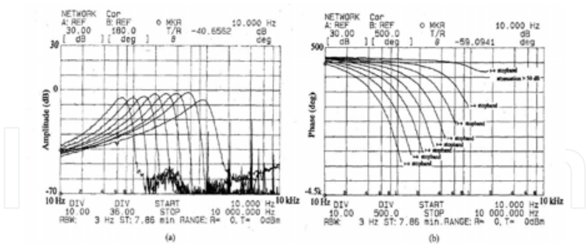
Fig. 17. Measured a) amplitude and b) phase responses from 8 taps of a 32-section SC filter-cascade; from Bor (Bor and Wu, 1996).
