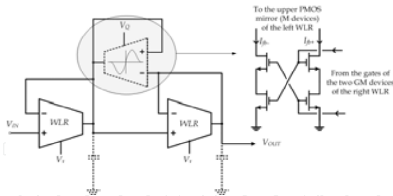
Fig. 19. A schematic block diagram of the fuse biquad. The dotted components indicate that they are not explicitly implemented in the actual circuit topology. The voltages V_i and V_Q set the pole frequency \omega_0 and quality factor Q of the filter; adapted from Sarpeshkar (Sarpeshkar et al., 1996).
