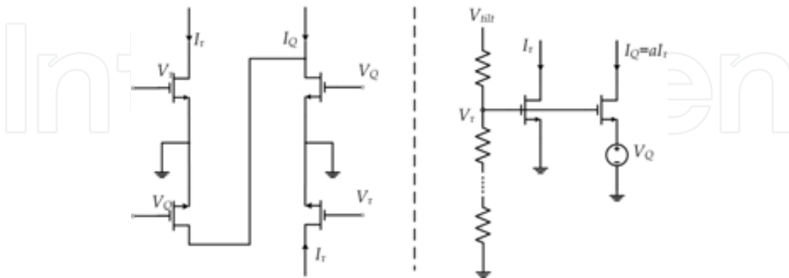
Fig. 10. The 'pseudo-quad' structure, formed by duplicating the Q bias transistor and juxtaposing the resulting pair with the \tau bias transistors (left). Q -source control by externally providing a voltage V_Q to scale the feedback amplifier current I_Q with respect to I_\tau (right); adapted from Watts (Watts et al., 1992).
