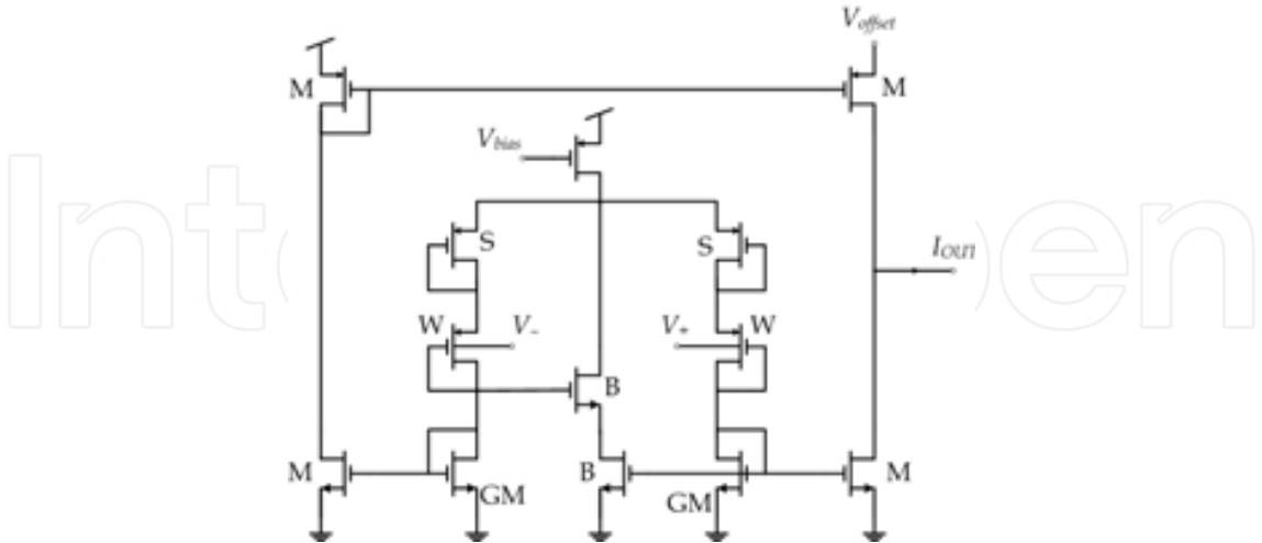
Fig. 18. The WLR OTA. The devices marked S and GM denote the source and gate degeneration transistors, whereas the devices W and M denote the well-input and mirror transistors. The B transistors perform bump linearization. In addition, the voltage V_{bias} sets the bias current of the amplifier, whereas V_{offset} allows fine adjustment of the amplifier’s output offset if necessary; adapted from Sarpeshkar (Sarpeshkar et al., 1996).
