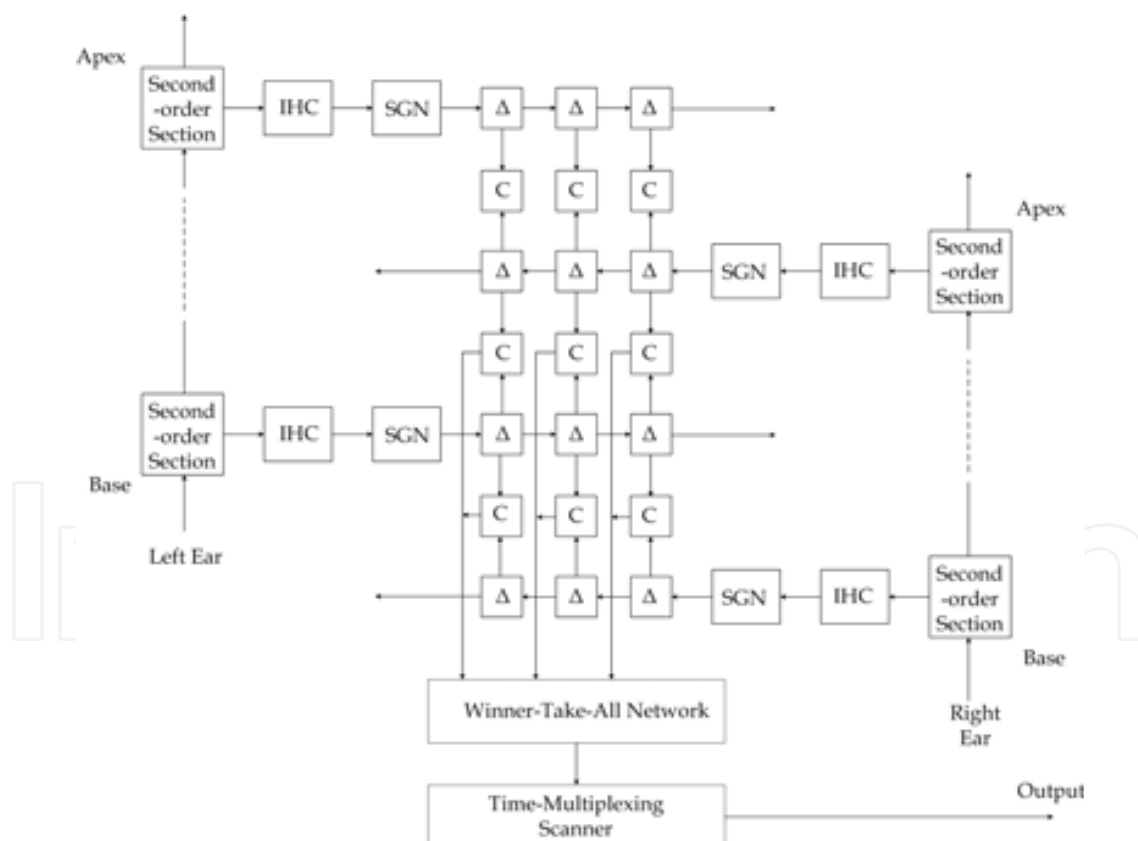
Fig. 8. Floorplan of the silicon model for sound localization of the owl. The square blocks marked with a ' \Delta ' represent the discrete delay elements forming the silicon axons, whereas the square blocks marked ' C ' in between every antiparallel axon are the correlators or coincidence detectors which take two inputs from the upper and lower axons; adapted from Lazzaro (Lazzaro and Mead, 1990).
