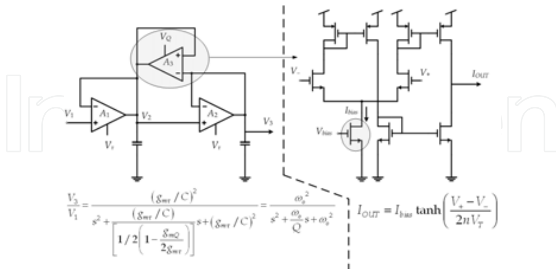
Fig. 3. The lowpass biquad circuit. The \omega_o and Q control inputs set the OTA bias currents for controlling the pole frequency and quality factor (and hence the peak gain) of the filter response. Amplifiers A_1 and A_2 have the same transconductance gm (left). The basic CMOS OTA circuit used for realizing amplifiers A_1 , A_2 and A_3 (right). The implemented relations are shown beneath each circuit. Parameters V_T and n denote the thermal voltage and subthreshold slope parameter, respectively; adapted from Lyon (Lyon and Mead, 1988a).
