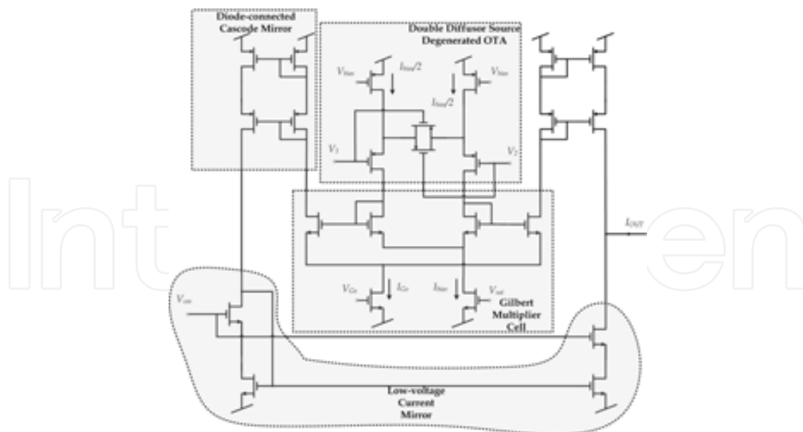
Fig. 22. Furth's wide linear range OTA implementation. The voltage V_{G0} sets the gain of the Gilbert Multiplier Cell, V_{sat} is the biasing of the level shifter transistor, whereas V_{cas} is the biasing of the low-voltage current mirror; adapted from Furth (Furth and Andreou, 1996b).
