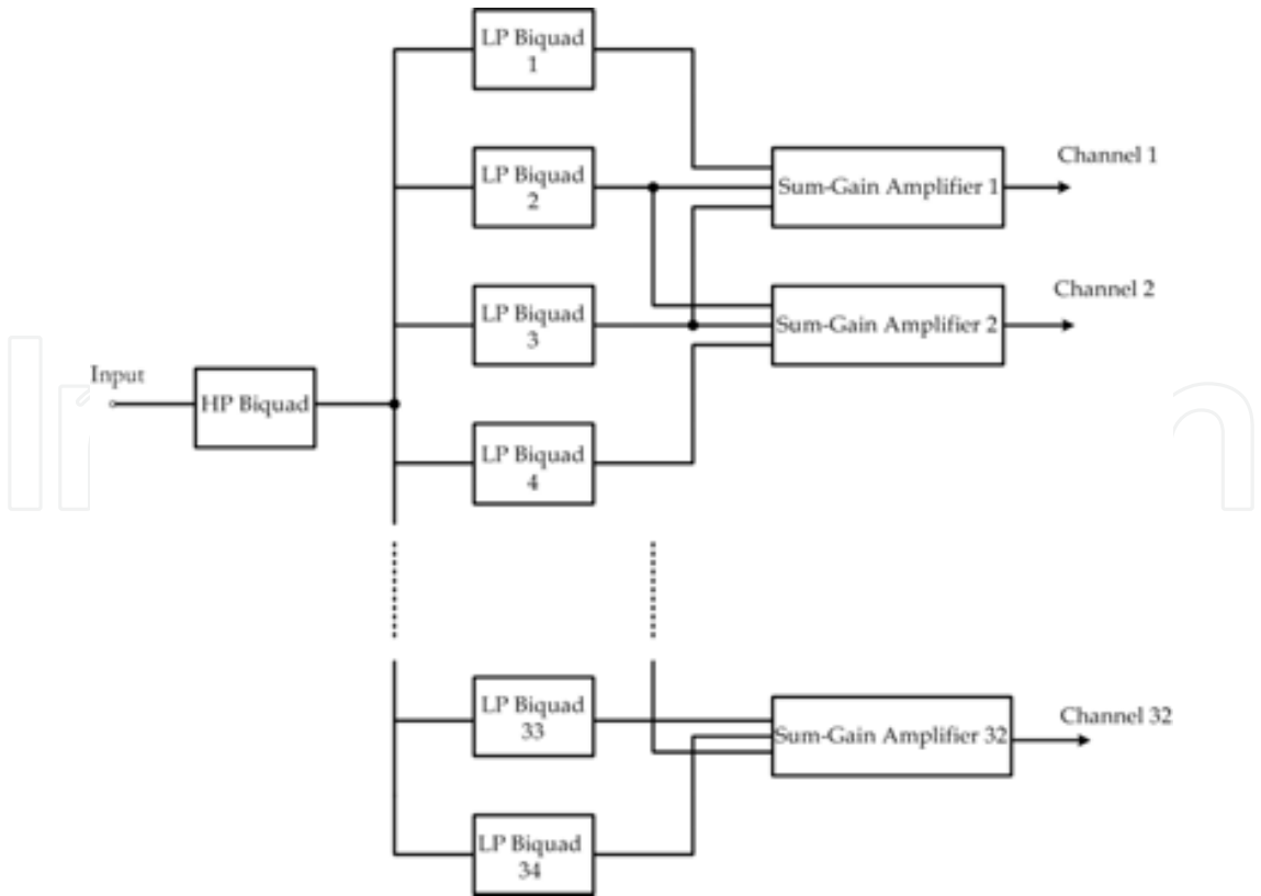
Fig. 13. Dilating-biquads filterbank; adapted from Lin (Lin et al., 1992a).
