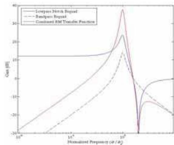
Fig. 2. Indicative transfer functions of the LPN, resonator and their combined response resembling the one obtained from a particular output tap.
