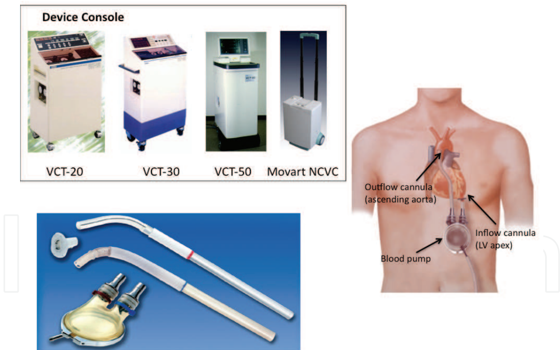
Fig. 1. Toyobo-LVAS® system. Different types of devise console ( left upper panel ); blood pumps and inflow/outflow cannula ( left lower panel ); and the chart of LVAD system ( right panel ). The blood pump was consisted of diaphragm with pulsatile flow through two mechanical valves, operated by pneumatic driven system. The maximum stroke volume was 70 mL per bear under testing with water. Material of blood contacting surface is covered by segmented-polyurethane for medical use.
