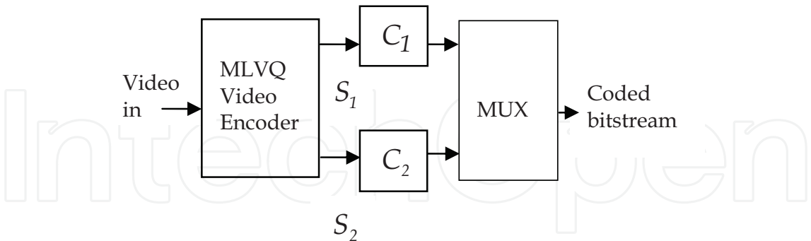
Fig. 10. UEP scheme for MLVQ video codec
