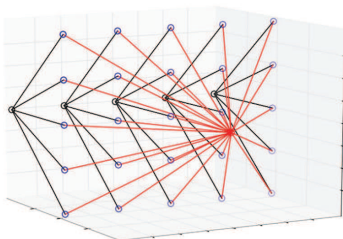
Fig. 5. A simplified ESNN structure
