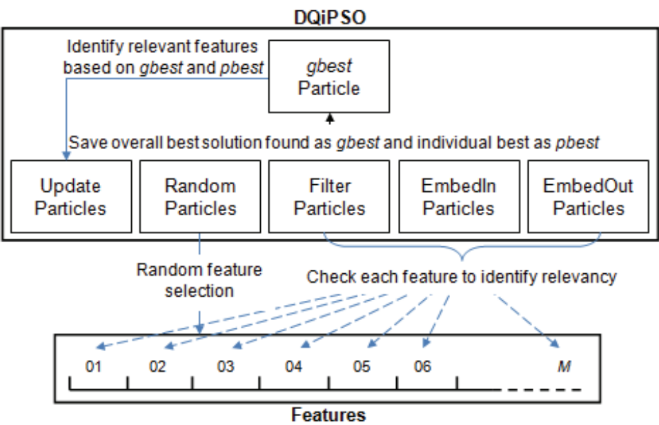
Fig. 2. DQiPSO feature selection strategy
