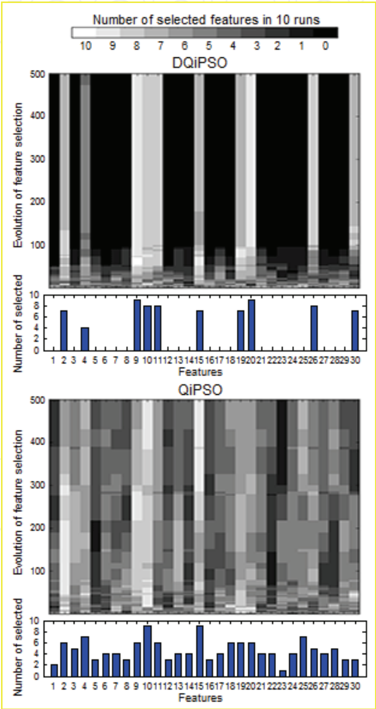
Fig. 7. Evolution of feature selection
