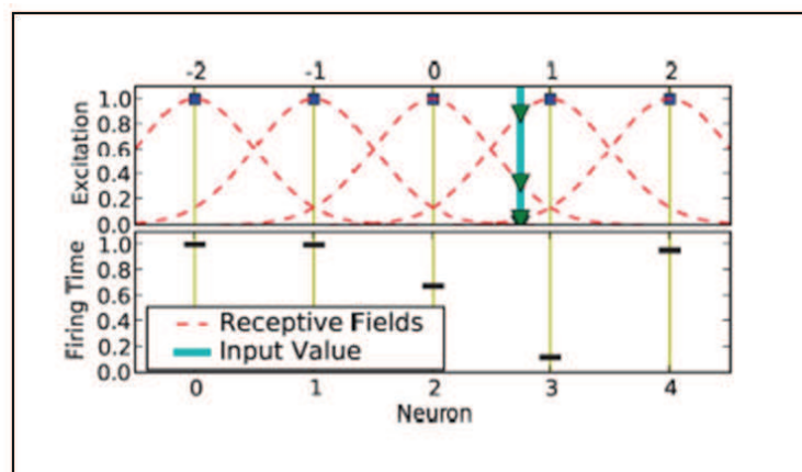
Fig. 4. Population Encoding Method.
