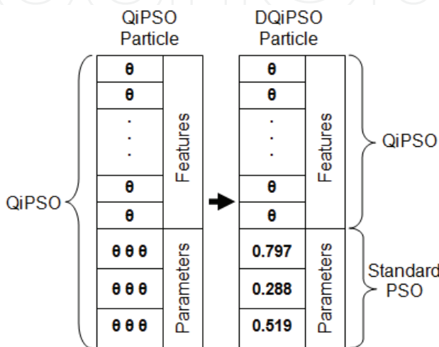
Fig. 1. The proposed hybrid particle structure in DQiPSO
