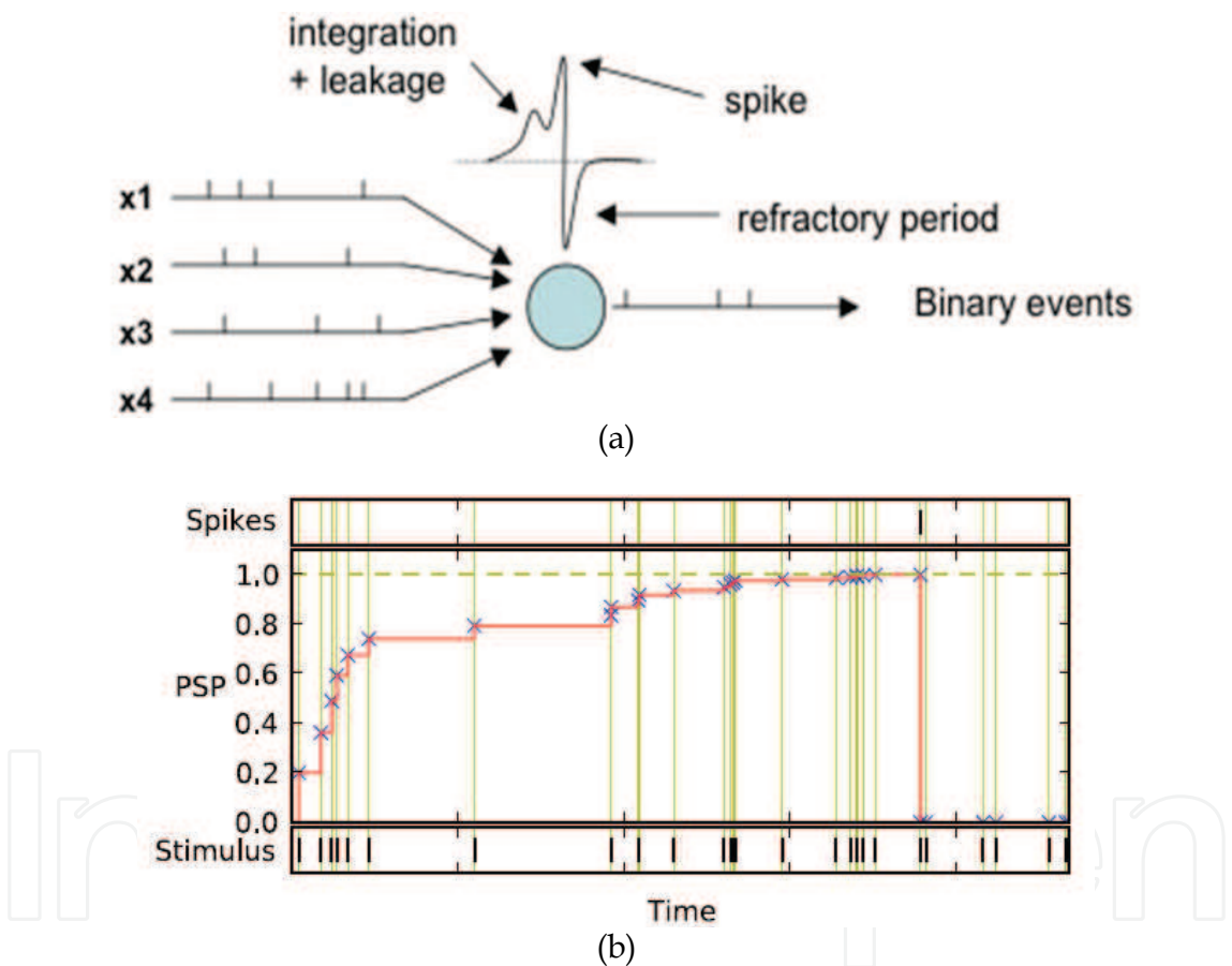
Fig. 3. (a) A simplified diagram of a spiking neuron model. (b) A spiking neuron emits an output spike when the total spiking input – Post Synaptic Potential (PSP), is larger than a spiking threshold. Based on the SNN, Evolving SNN (ESNN) was introduced (Wysoski et al., 2006) where SNN evolve their structure through fast one-pass learning from data and have the potential for solving complex problems. ESNN have been applied for classification tasks, such as face recognition, person authentication based on audiovisual information, taste recognition. They achieved better results than previously published models. The ESNN architecture consists of an encoding method for real value data to spike time, neuron model and learning method.
