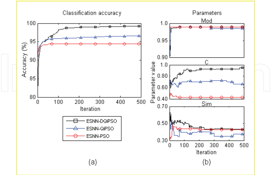
Fig. 8. a) Classification accuracy and b) Parameter optimization result
