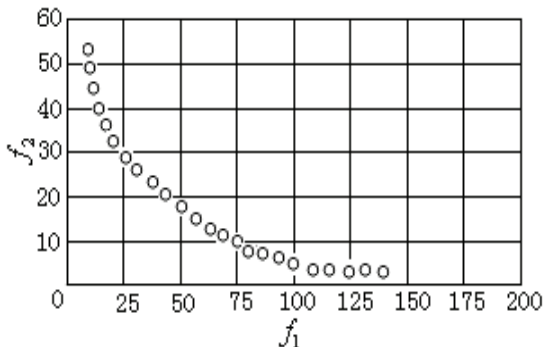
Fig. 5. Pareto front on BNH using LEA
