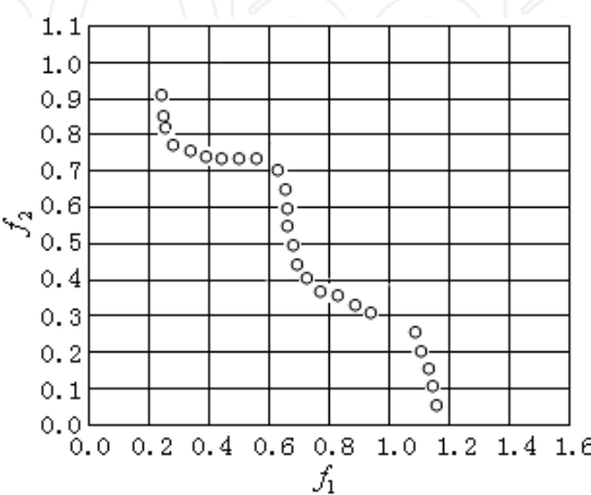
Fig. 7. Pareto front on TNK using LEA
