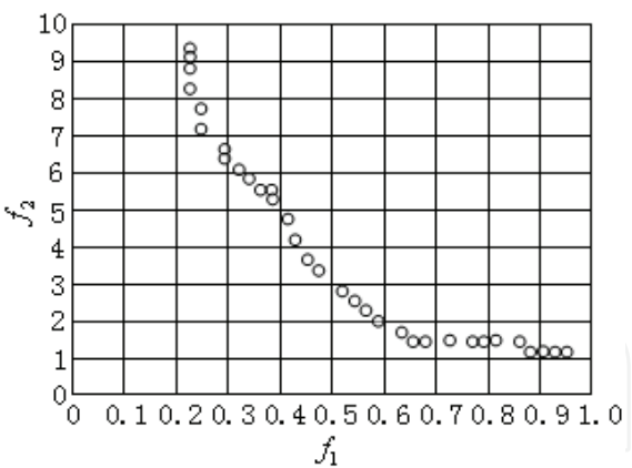
Fig. 9. Pareto front on CE using LEA
