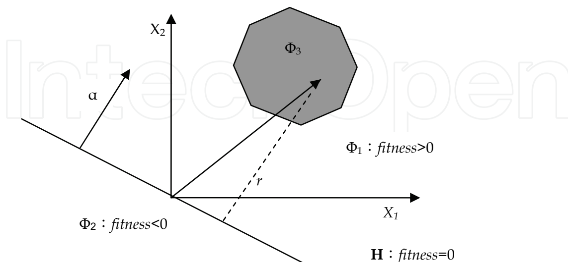
Fig. 3. Transformation of searching space.
