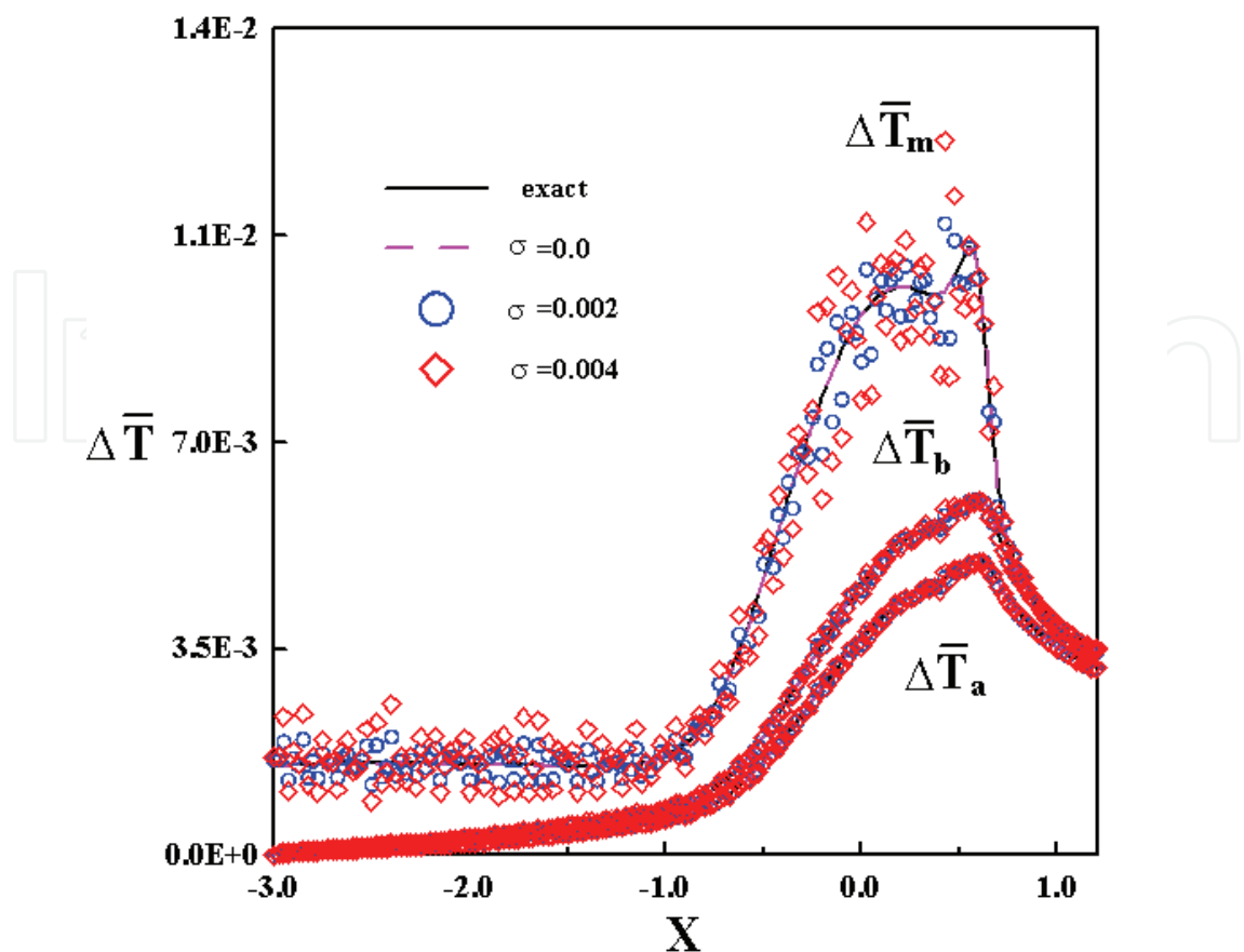
Fig. 5. Temperature rise distributions for different standard deviations of the measured errors with 169 measured points in the film thickness using direct inverse method.
