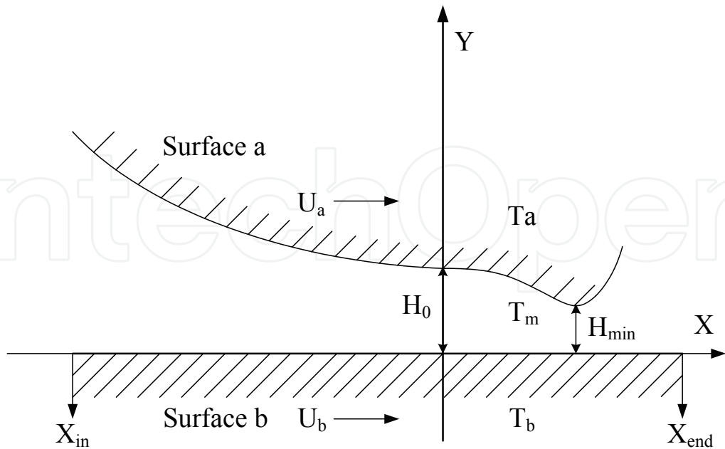
Fig. 1. The geometry of an EHL line contact.
