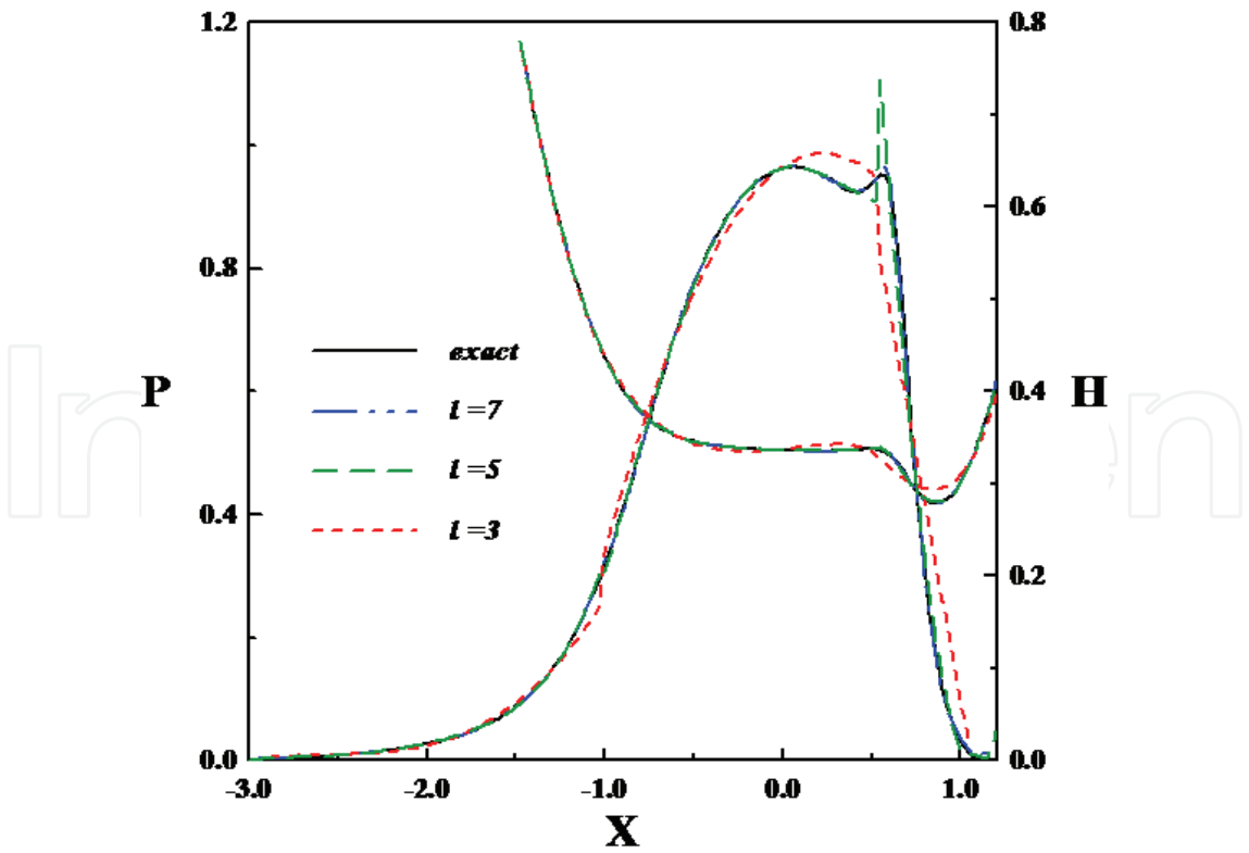
Fig. 8. Pressure distributions and film shapes for different degrees with 31 measured points in the film thickness using inverse approach.
