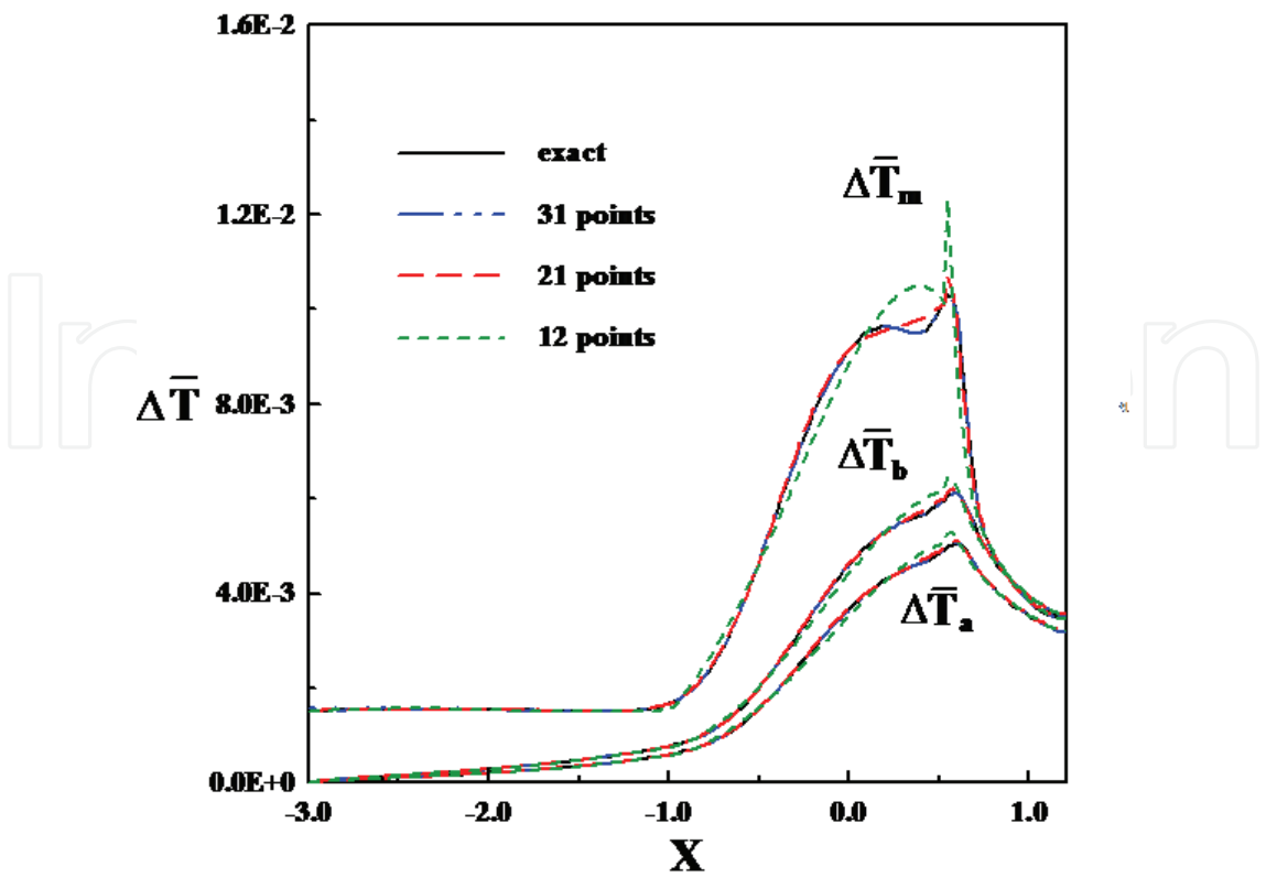
Fig. 7. Temperature rise distributions for different measured points in the film thickness using inverse approach.
