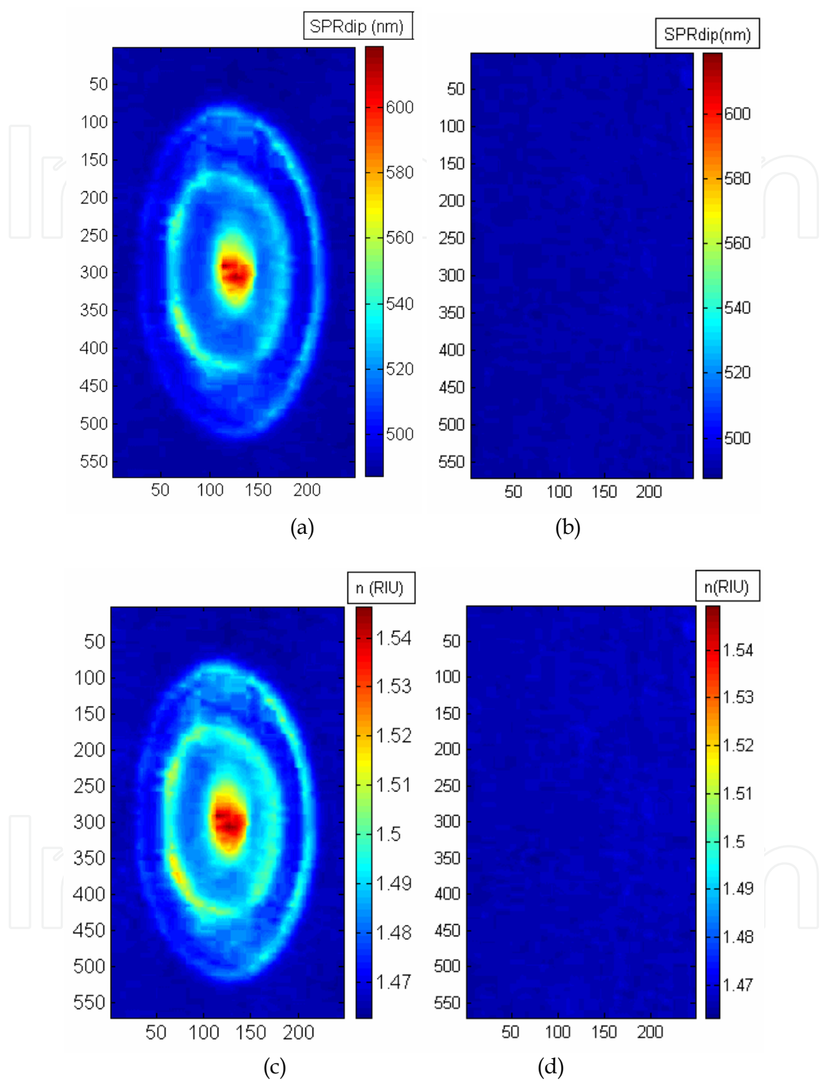
Fig. 8 a) SPR wavelength minimum profile of lubricant PB 2400 dimple b) SPR wavelength minimum profile of control image c) Refractive index profile of lubricant PB 2400 dimple d) Refractive index profile of control image.
