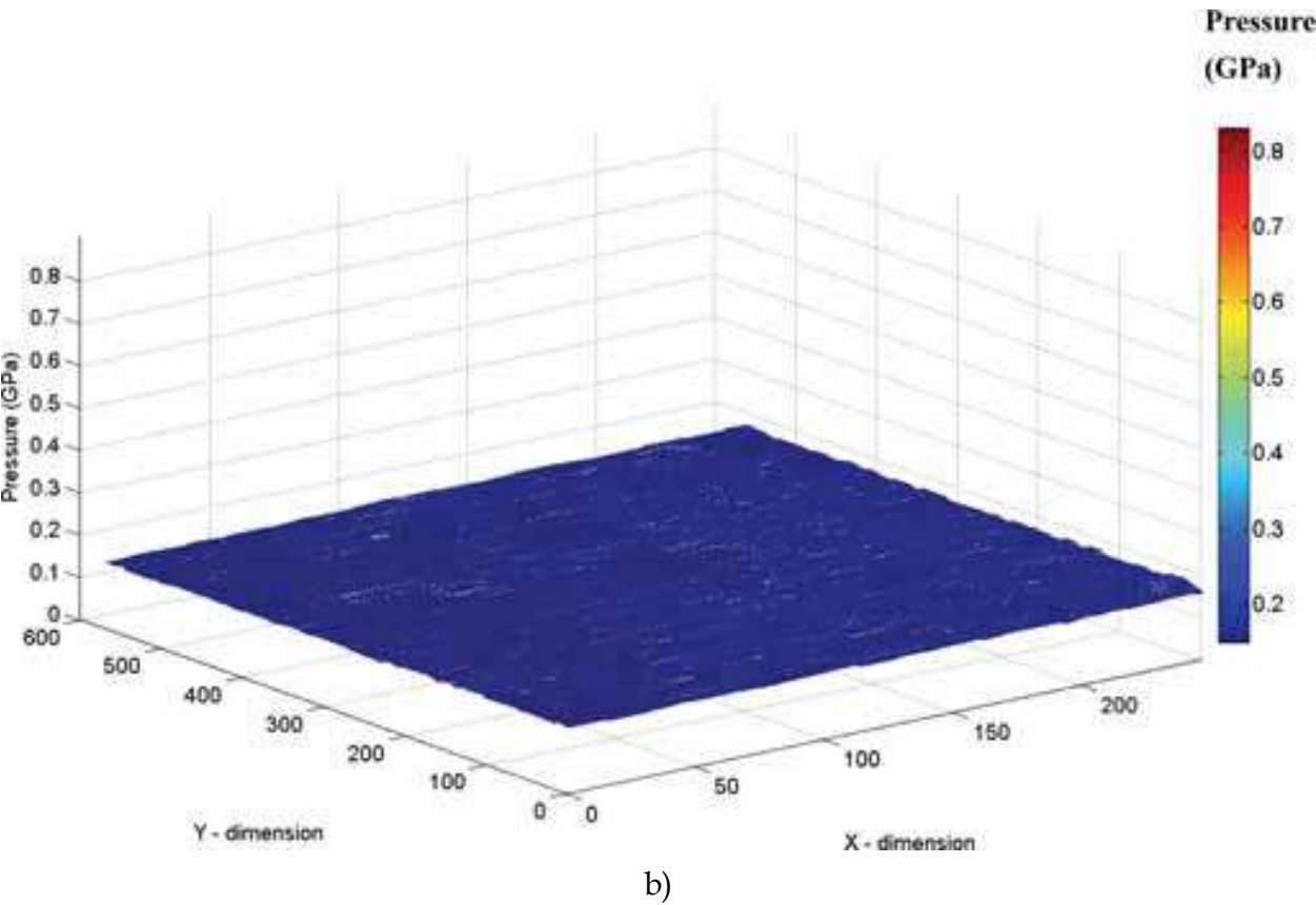
Fig. 10. a) Pressure profile of lubricant PB 2400 dimple, b) Pressure profile of control image.
