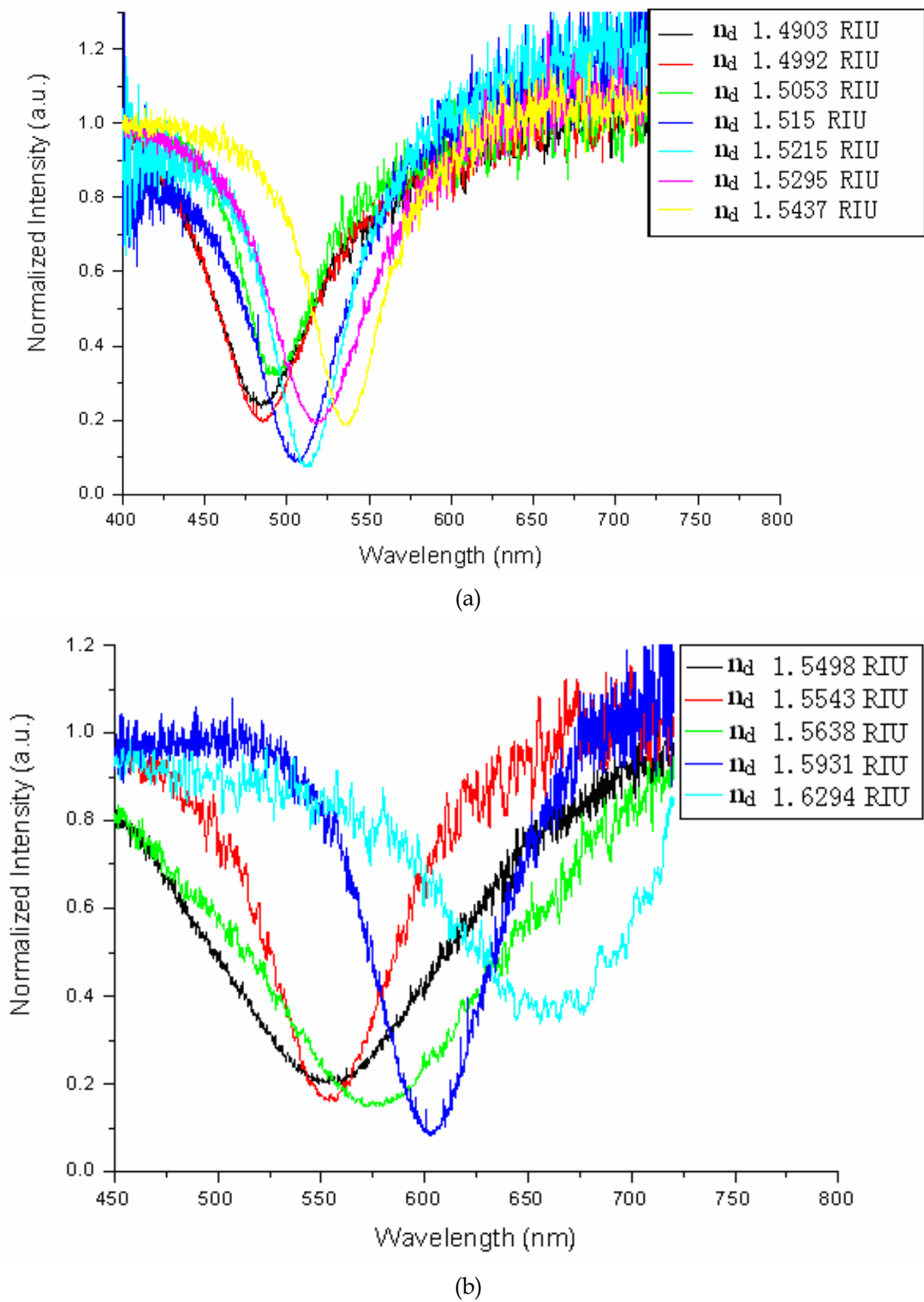
Fig. 6. SPR absorption spectra of lubricant samples for calibration.
