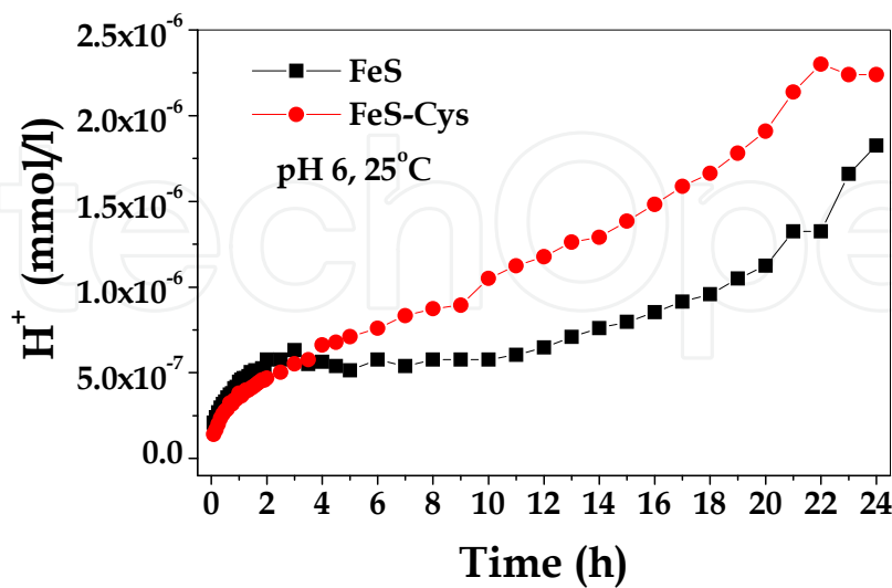
Fig. 17. [H^+] concentration during the mackinawite oxidation process (long time), starting after pH maximum.
