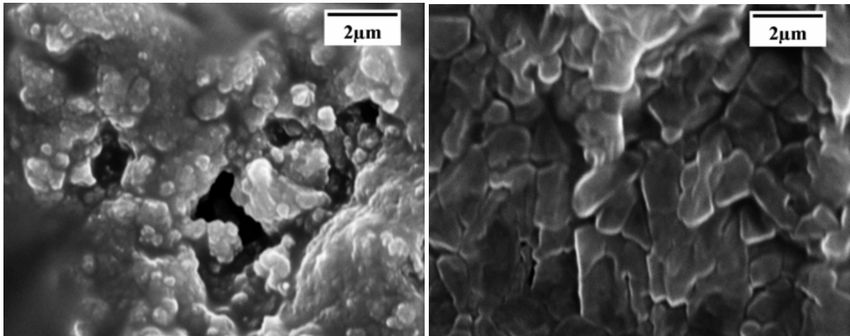
Fig. 8. Scanning Electron Microscopy: a) unmodified mackinawite; b) modified mackinawite. (10,000 x magnification).
