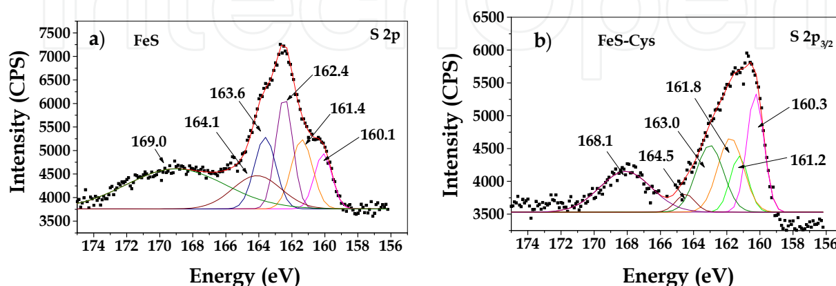
Fig. 4. XPS spectra of S 2p: a) FeS and b) FeS-Cys – Errors for energy \pm 0.3 eV.
