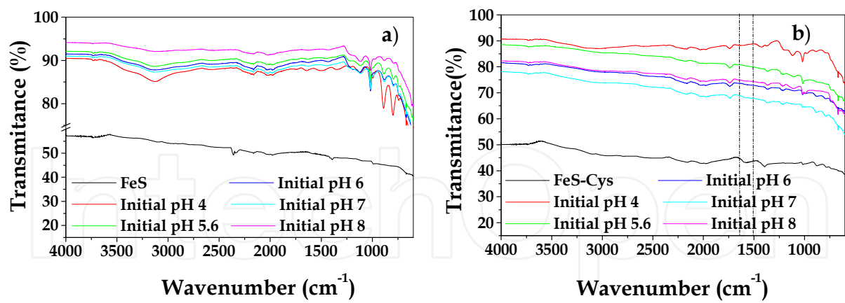
Fig. 13. FTIR spectra of a) unmodified and b) modified mackinawite after oxidation processes (short time)
