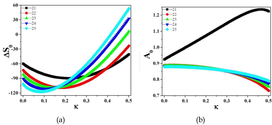
Fig. 3. Influence of the WDR, \kappa , on the dynamics of sediment transport: (a) the QES, \Delta S ; (b) the positive part of SCC, A_0
