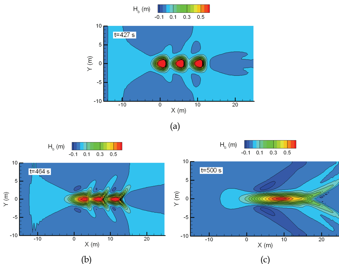
Fig. 12. Evolution of sand dunes (seabed elevation)
