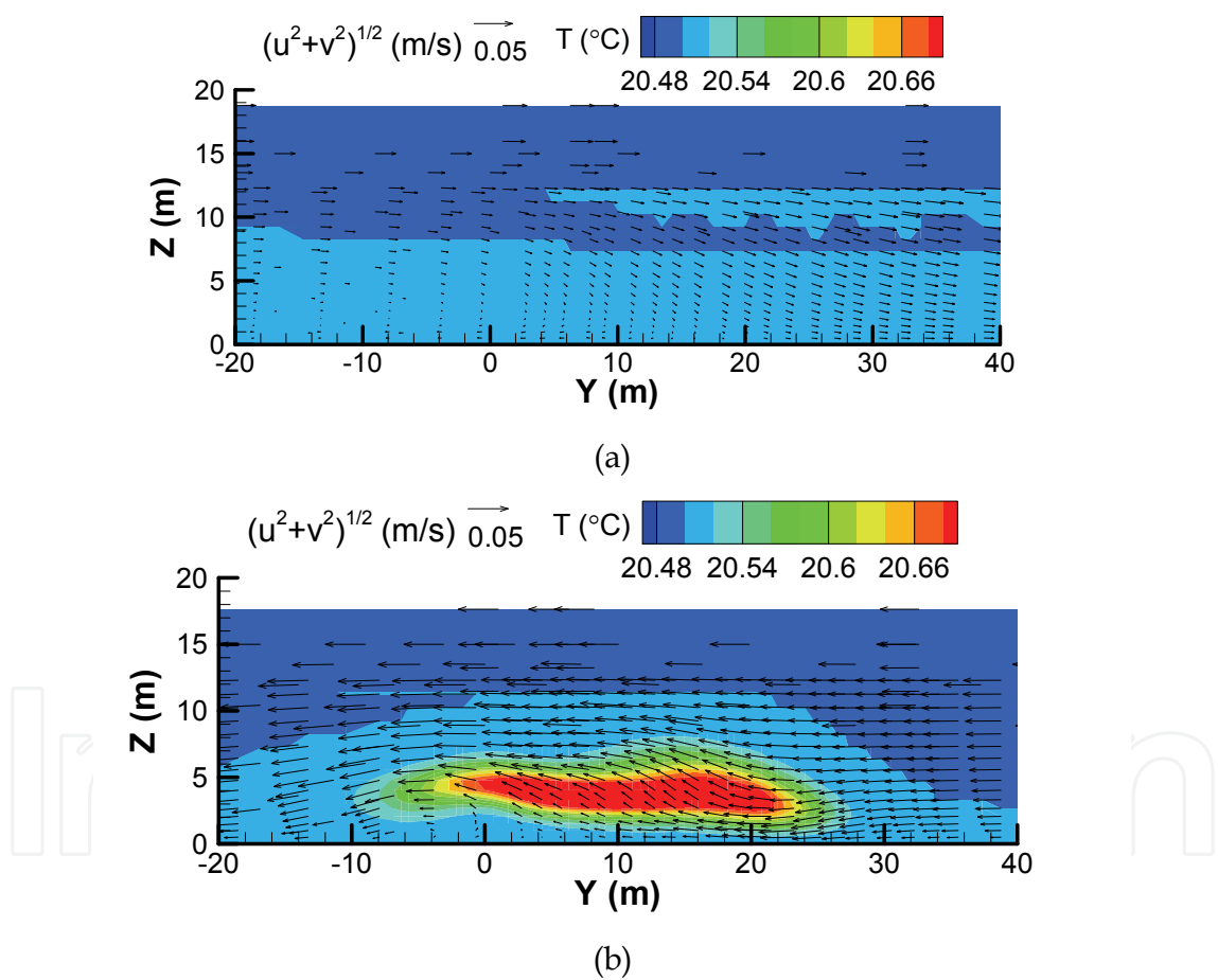
Fig. 8. Cross-section velocity and temperature at 10 m downstream from the diffuser in the x direction. (a) Flood tide. (b) Ebb tide.
