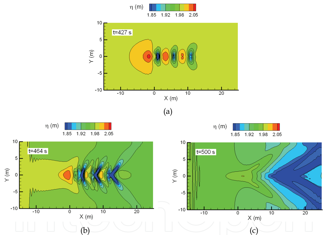
Fig. 13. Evolution of water surface elevation
