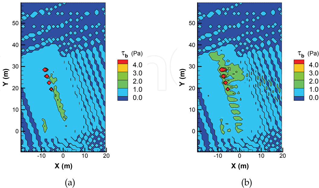
Fig. 10. Bottom drag calculated from Eq. (11). (a) Flooding tide; maximum shear stress is 165.83 \text{ Pa} . (b) Ebb tide; maximum shear stress is 169.59 \text{ Pa} .
