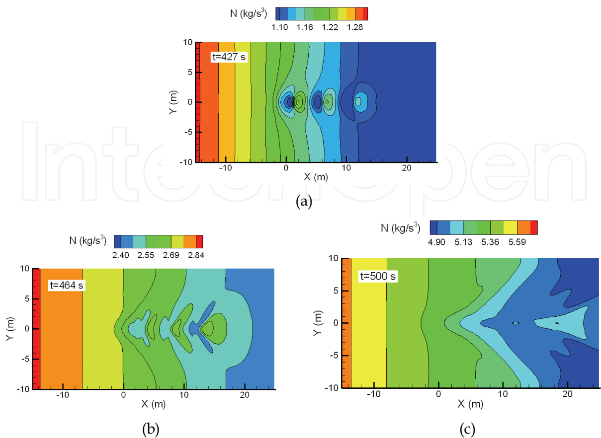
Fig. 14. Evolution of wave action
