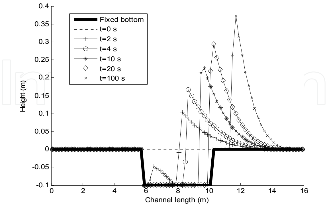
Fig. 7. Bed evolution in the hypothetical test case.
