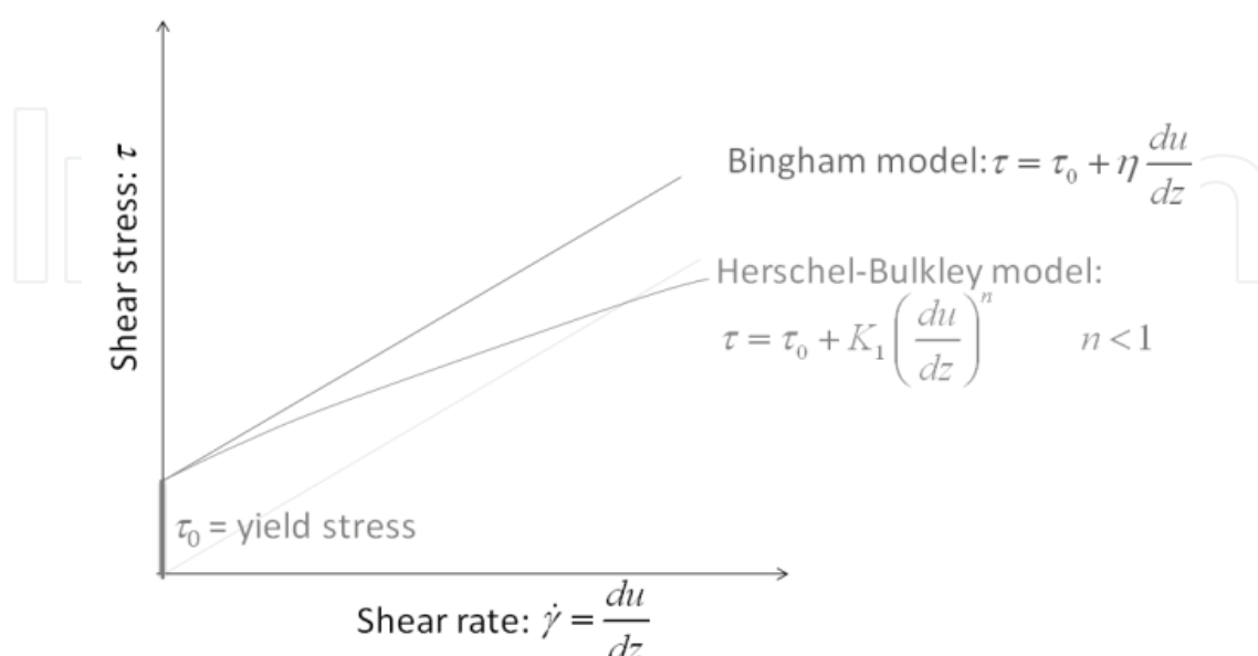
Fig. 9. Shear stress as a function of shear rate for yield stress fluids.
