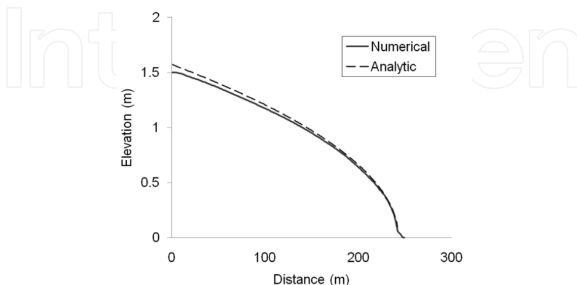
Fig. 10. Numerical predictions (Bingham model) vs. analytical solution for the slump test.
