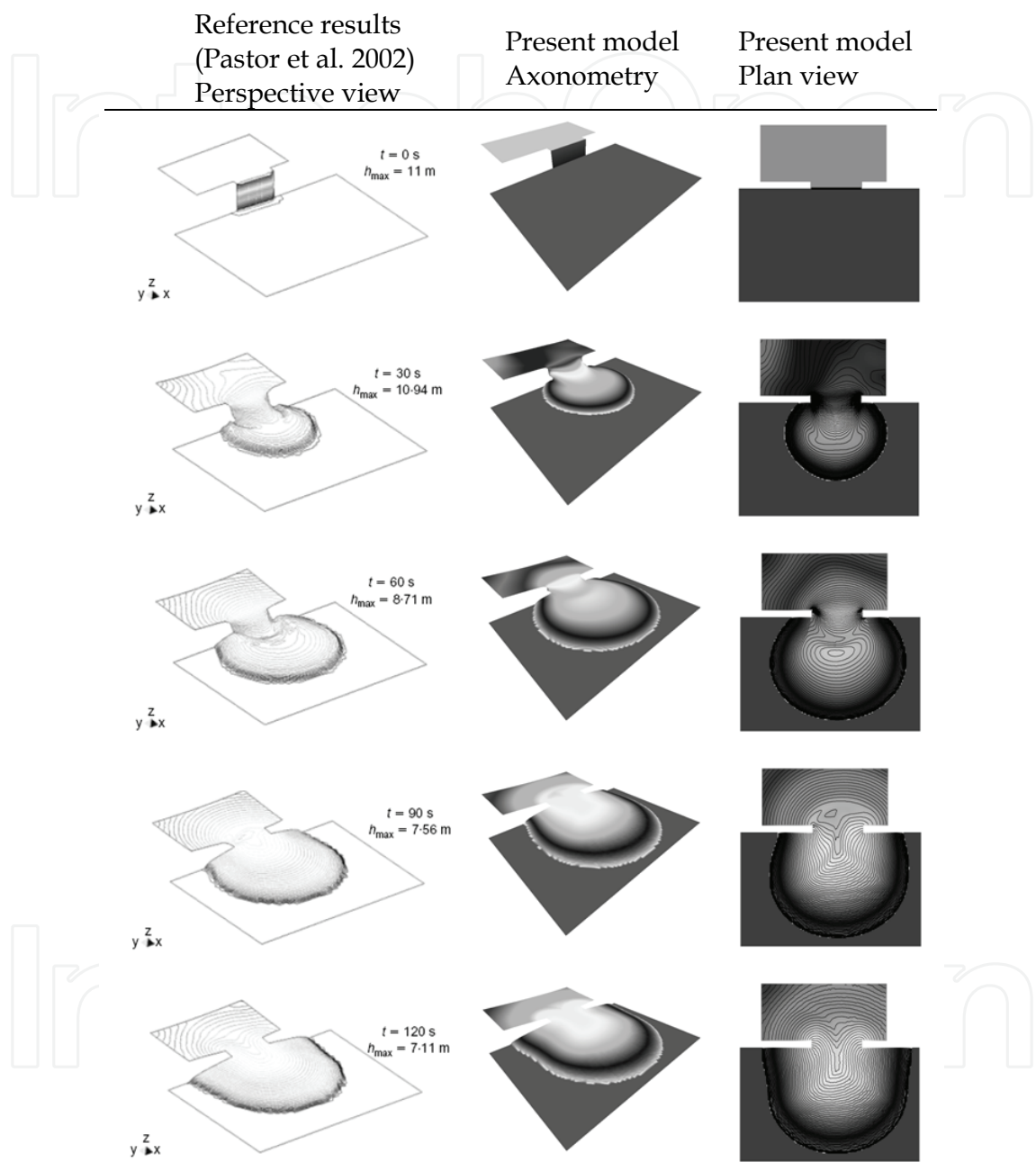
Fig. 11. Reference results in perspective (left), axonometric view and plan view of predictions of the model developed here for the “Gypsum dam” collapse.
