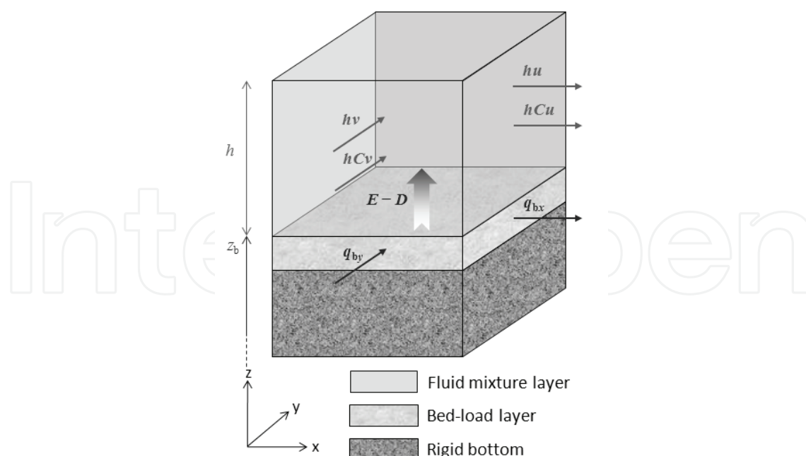
Fig. 2. Schematic configuration underlying the depth-averaged morphodynamic model.
