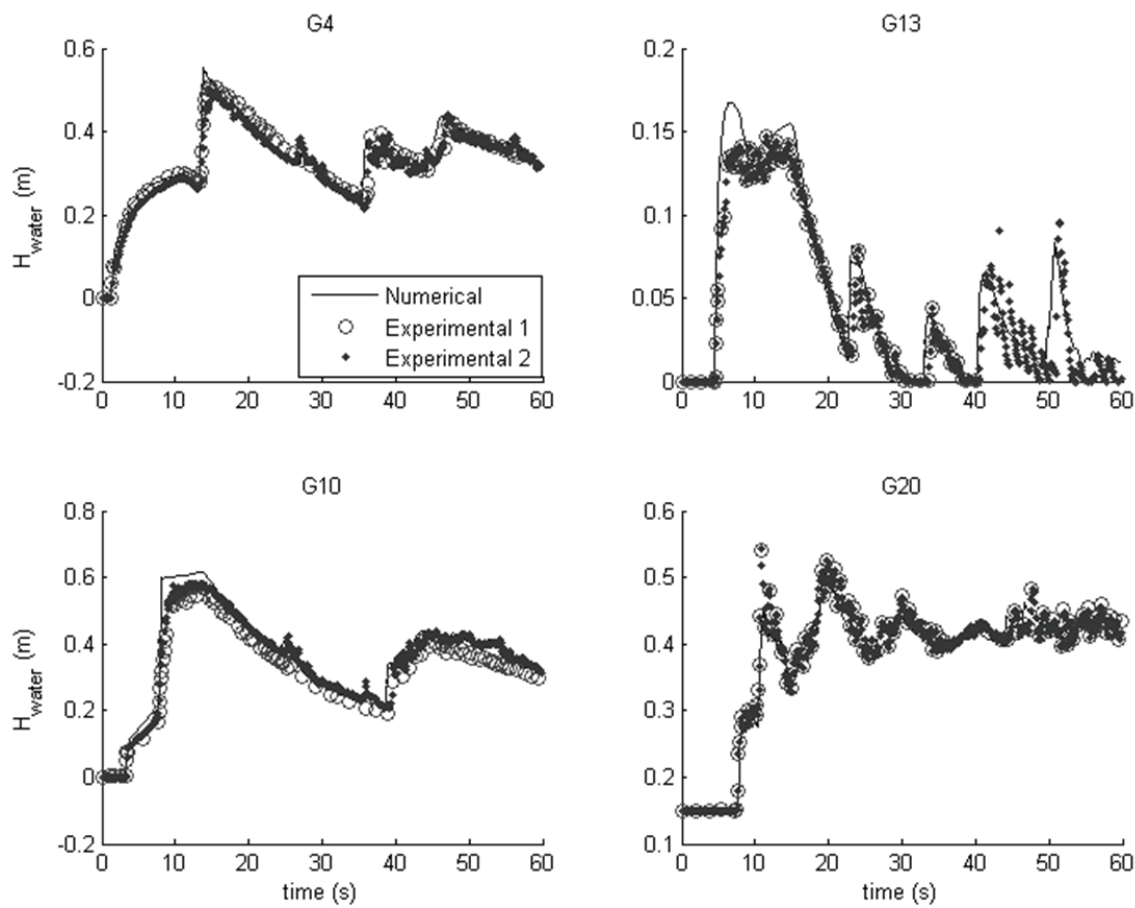
Fig. 6. Evolution of the water depth at gauges.
