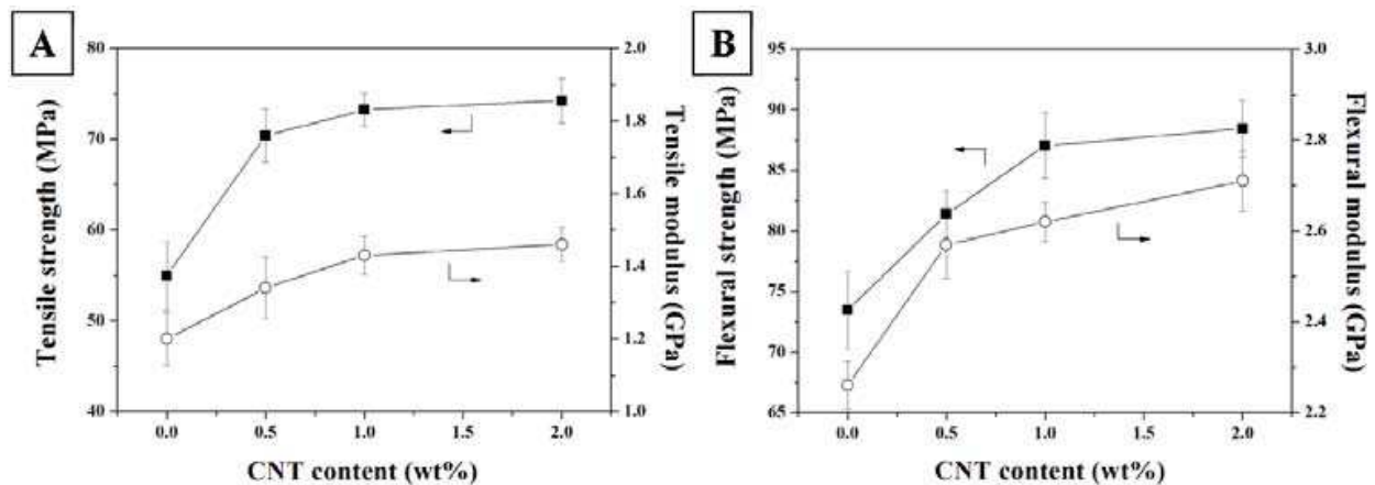
Fig. 7. Variations of (A) tensile strength and tensile modulus and (B) flexural strength and flexural modulus of PBT nanocomposites with the CNT content. Reproduced with permission from Ref. (Kim, 2009b). © 2009 Wiley Periodicals, Inc.
