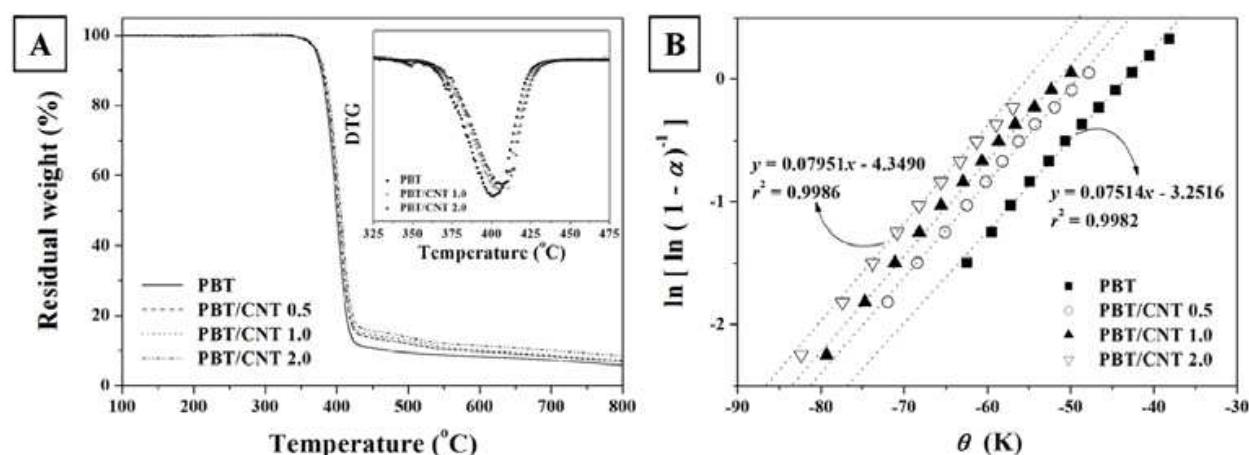
Fig. 11. (A) TGA thermograms of PBT nanocomposites. (B) Plots of \ln[\ln(1 - \alpha)^{-1}] versus \theta as shown for PBT nanocomposites. Reproduced with permission from Ref. (Kim, 2009b). © 2009 Wiley Periodicals, Inc.
