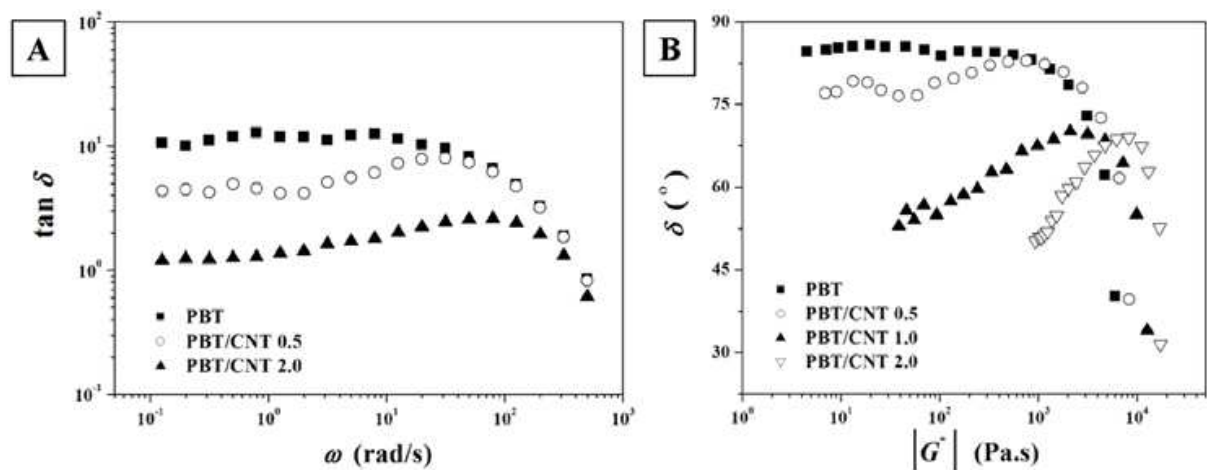
Fig. 3. (A) Variations of \tan \delta of PBT nanocomposites as a function of frequency. (B) Plots of the phase angle ( \delta ) versus the complex modulus ( |G^*| ) of PBT nanocomposites. Reproduced with permission from Ref. (Kim, 2009b). © 2009 Wiley Periodicals, Inc.
