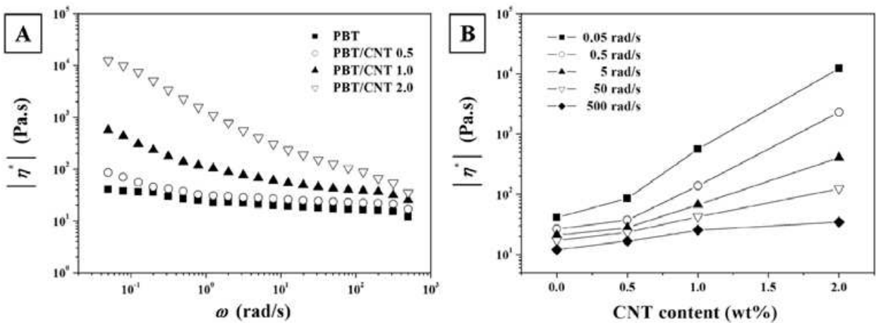
Fig. 1. (A) Complex viscosity ( |\eta^*| ) of PBT nanocomposites as a function of frequency. (B) Variations of |\eta^*| of PBT nanocomposites with the CNT content at different frequencies. Reproduced with permission from Ref. (Kim, 2009b). © 2009 Wiley Periodicals, Inc.
