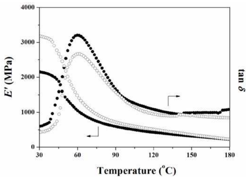
Fig. 5. Dynamic mechanical properties of PBT nanocomposites as a function of temperature. Filled and open circles represent the values of E' and \tan \delta for pure PBT and PBT/CNT 2.0 nanocomposites. Reproduced with permission from Ref. (Kim, 2009b). © 2009 Wiley Periodicals, Inc.
