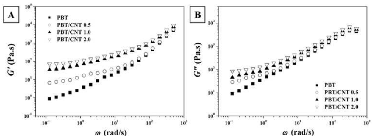
Fig. 2. (A) Storage modulus ( G' ) and (B) loss modulus ( G'' ) of PBT nanocomposites as a function of frequency. Reproduced with permission from Ref. (Kim, 2009b). © 2009 Wiley Periodicals, Inc.
