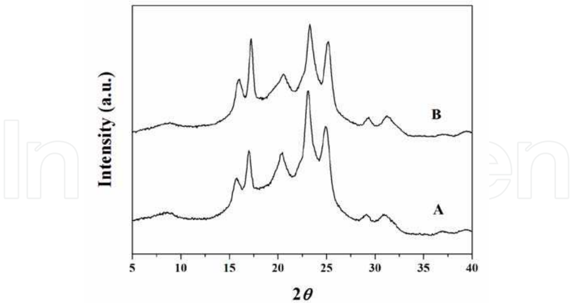
Fig. 10. Wide-angle X-ray diffraction (WAXD) patterns of (A) pure PBT and (B) PBT/CNT 2.0 nanocomposites. Reproduced with permission from Ref. (Kim, 2009b). © 2009 Wiley Periodicals, Inc.
