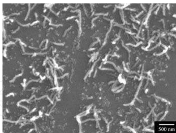
Fig. 12. SEM micrograph of the residues of PBT/CNT 2.0 nanocomposites after the thermal decomposition process. Reproduced with permission from Ref. (Kim, 2009b). © 2009 Wiley Periodicals, Inc.
