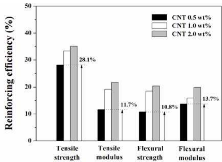
Fig. 8. Reinforcing efficiency of CNT on the mechanical properties of PBT nanocomposites. Reproduced with permission from Ref. (Kim, 2009b). © 2009 Wiley Periodicals, Inc.
