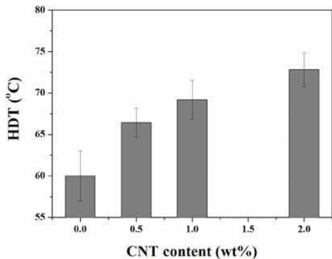
Fig. 9. Heat distortion temperature (HDT) of PBT nanocomposites. Reproduced with permission from Ref. (Kim, 2009b). © 2009 Wiley Periodicals, Inc.
