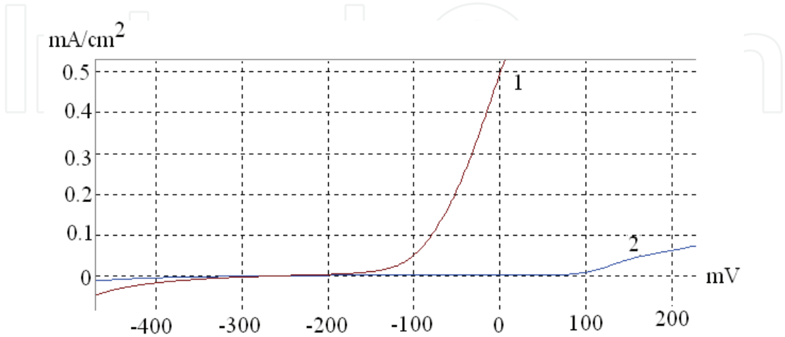
Fig. 8. Polarization curves – Overlapping: Ni/ZrO 2 in Na 2 SO 4 0.1 M solution (1), Ni/ZrO 2 in NaCl 3% solution (2) In figure 9, the polarization curve is shown for nickel and Ni/ZrO 2 specimens in H 2 SO 4 0.1 N solution. The curve for nickel has a maximum peak at a voltage E \in (7\text{mV}, 14 \text{ mV}) and a corrosion rate i_{cor} \in (2.150 \text{ }\mu\text{A/cm}^2, 2.154 \text{ }\mu\text{A/cm}^2) . For Ni/ZrO 2 two maximum peaks are present at a voltage E_1 \in (-65 \text{ mV}, -55 \text{ mV}) , a corrosion rate i_{cor 1} \in (4 \text{ }\mu\text{A/cm}^2, 4.2 \text{ }\mu\text{A/cm}^2) , and at a voltage E_2 \in (80 \text{ mV}, 100 \text{ mV}) , with a corrosion rate i_{cor 2} \in (2.3 \text{ }\mu\text{A/cm}^2, 2.5 \text{ }\mu\text{A/cm}^2) . In addition, we juxtaposed the polarization curves for Ni/ZrO 2 in H 2 SO 4 0.1 N solution (1), and Ni in H 2 SO 4 0.1 N solution (2). Both curves have a peak in the same voltage range: E \in (-255 \text{ mV}, 200 \text{ mV}) .
