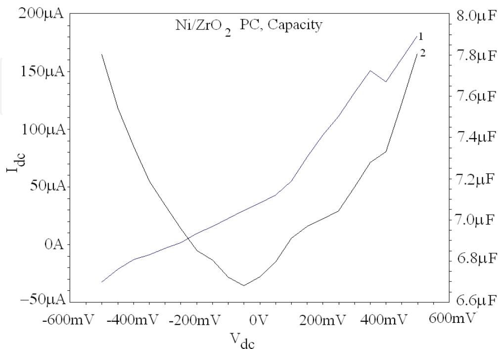
Fig. 15. Polarization curve (1) and variation of capacity (2) of nanocomposite thin films
