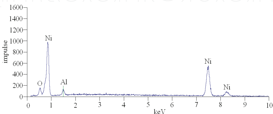
Fig. 3. EDAX spectrum of electrodeposited film with alumina nanoparticles
