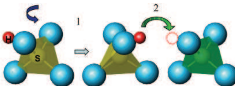
Fig. 6. Protons hopping in the Nafion membrane.
