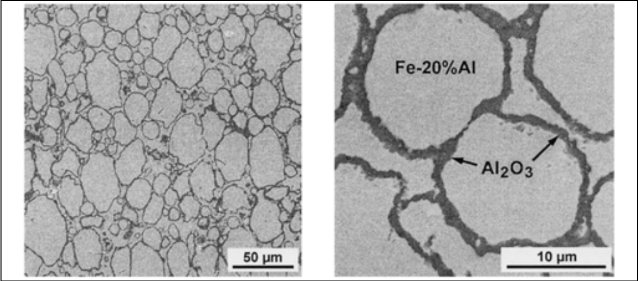
Fig. 18. SEM micrographs of an Fe 3 Al-20 vol.% Al 2 O 3 processed by an in situ displacement reaction via reactive sintering (Subramanian et al., 1998).
