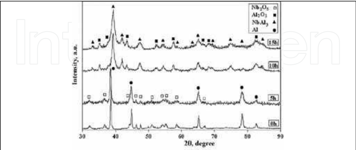
Fig. 20. XRD pattern of Nb 2 O 5 and Al powder mixture as-received and after different milling times (Mostaan et al., 2010b)
