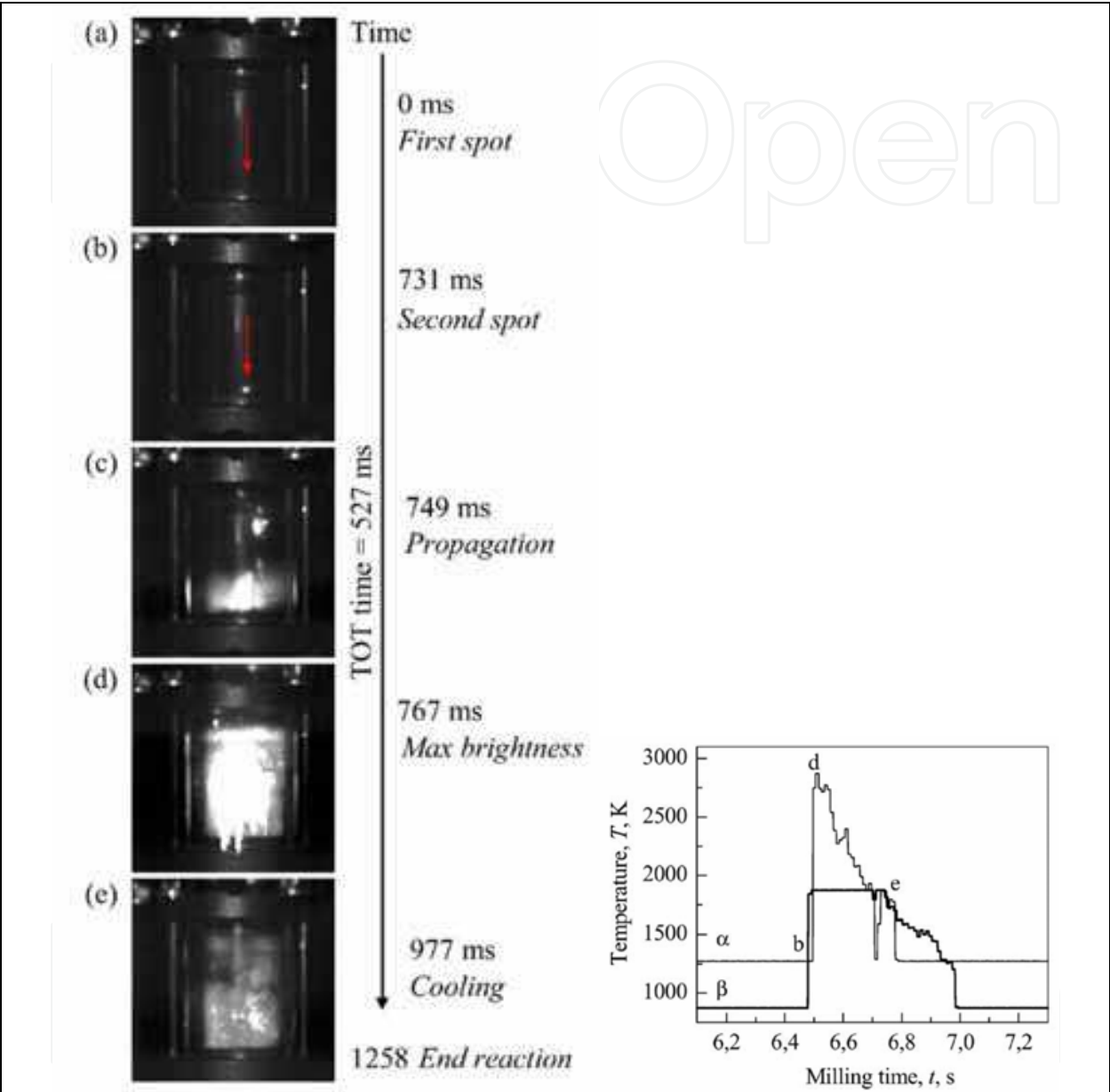
Fig. 3. High speed image sequence of the reaction of Ta:C=50:50 in a quartz vial coupled with the related temperature recording obtained by the infrared thermometer (Deidda et al., 2004). The modality of displacement reactions can be specified by theoretical adiabatic temperature, T_{ad} , of the reaction. T_{ad} represents the temperature of heat releasing during chemical reaction. A value of T_{ad}>1800\text{K} is generally considered to be the minimum necessary temperature for the occurrence of self-propagating combustion in a thermally ignited system (Munir, 1988). In contrast, Schaffer and McCormick (Schaffer & McCormick, 1990) showed that a value of T_{ad}>1300\text{K} is adequate for the sudden occurrence of chemical reaction during ball milling. The T_{ad} value could be estimated from the following relation:
