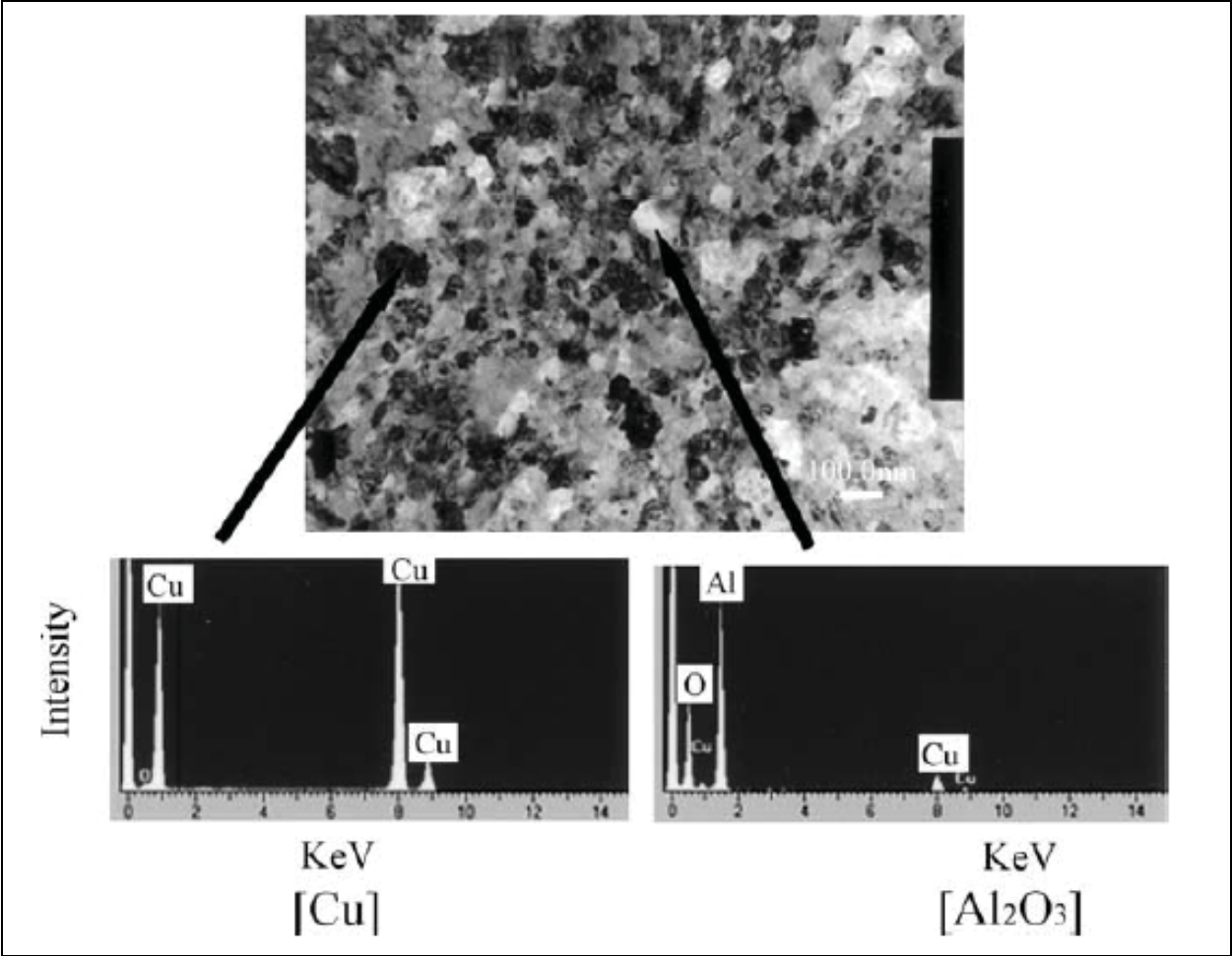
Fig. 6. TEM bright field image and energy dispersive spectroscopy (EDS) micrograph of the hot pressed Cu- 21 vol.% Al 2 O 3 sample (Hwang & Lee, 2005).
