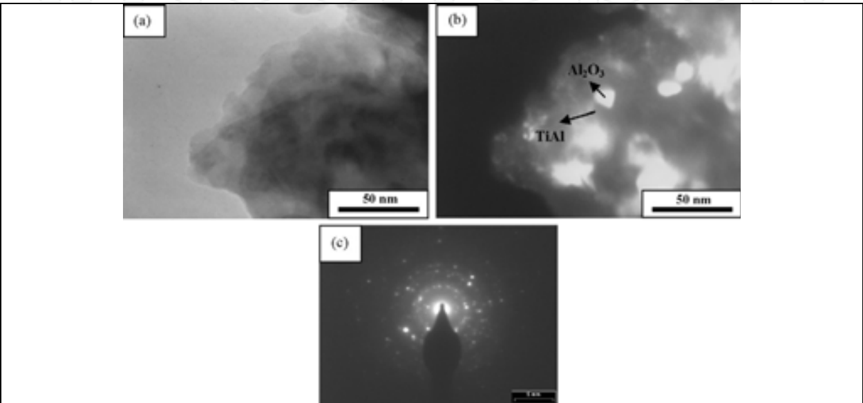
Fig. 19. TEM micrographs of TiAl-Al 2 O 3 nanocomposite powder produced by milling of TiO 2 +Al for 60 h followed by annealing at 900 °C: (a) Bright field, (b) Dark field, and (C) SAD pattern (Forouzanmehr et al., 2009).
