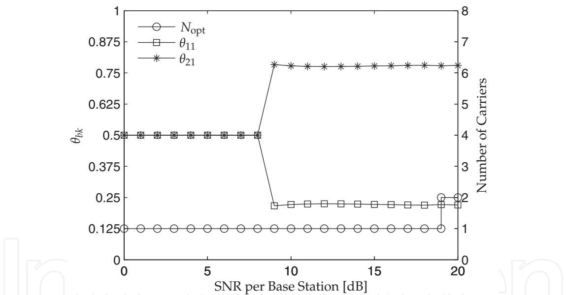
Fig. 10. Optimal values of \theta_{11} , \theta_{21} and N_{\text{opt}} for \gamma = [1, 3] bpcu and symmetric links
