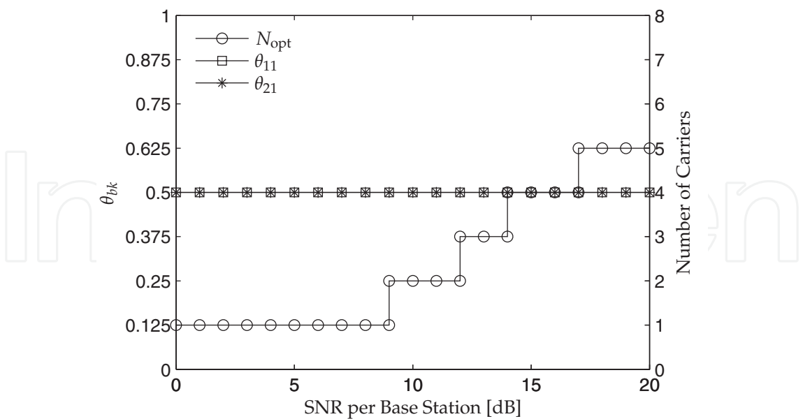
Fig. 9. Optimal values of \theta_{11} , \theta_{21} and N_{\text{opt}} for \gamma = [1, 1] bpcu and symmetric links
