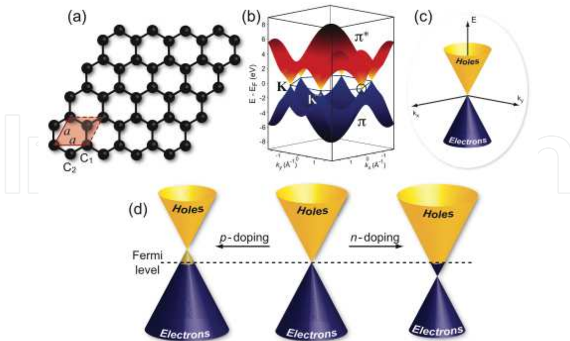
Fig. 1. (a) Crystal structure of the graphene layer where carbon atoms are arranged in the honeycomb lattice. Unit cell of graphene with lattice constant a has two carbon atoms per unit cell, C1 and C2. (b) Electronic dispersion of \pi and \pi^* states in the honeycomb lattice of free-standing graphene obtained in the framework of tight-binding approach. These branches have linear dispersion (c) in the vicinity of the K points of the Brillouin zone of graphene. (d) Position of the Dirac point and the Fermi level as a function of doping for the free-standing graphene.
