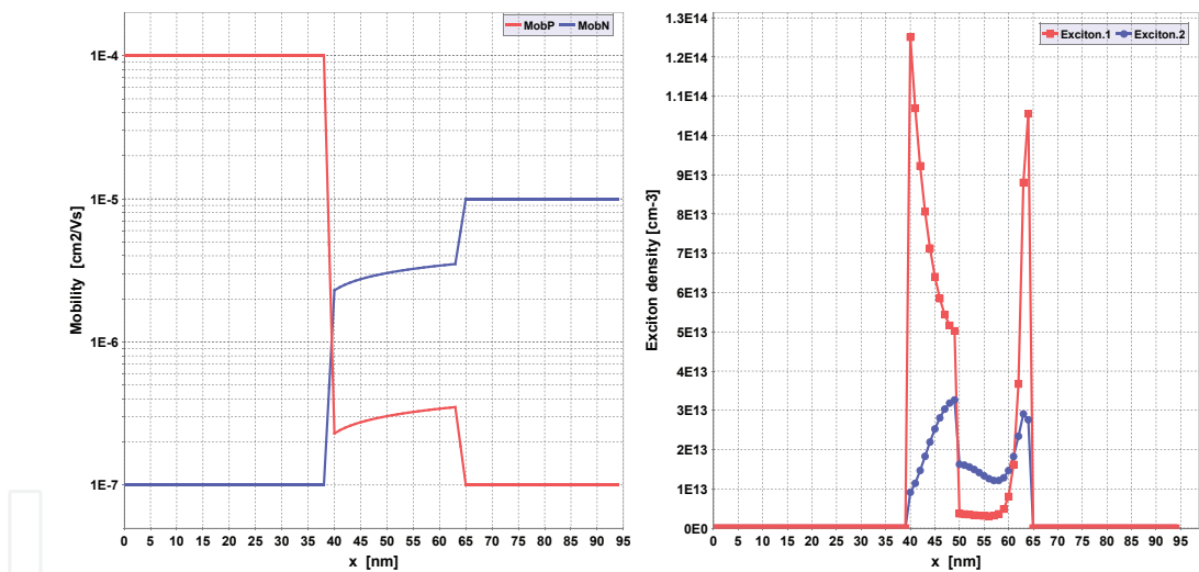
Fig. 10. Simulated profiles of mobilities (left) and Exciton.1 and Exciton.2 in the middle of the OLED structure (right).
