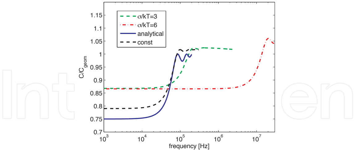
Fig. 7. Frequency dependence of the normalized capacitance at 6 V in a hole-only device for a constant mobility and diffusion coefficient, the EGDM and the analytical solution.
