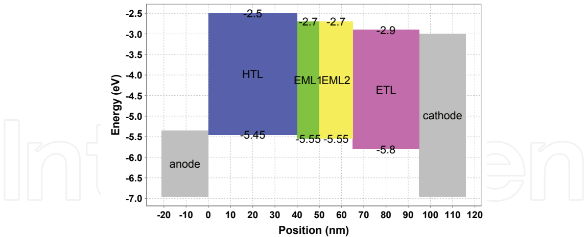
Fig. 8. Energy level diagram of a 4-layer OLED with two emissive layers EML1 and EML2 with two exciton species each.
