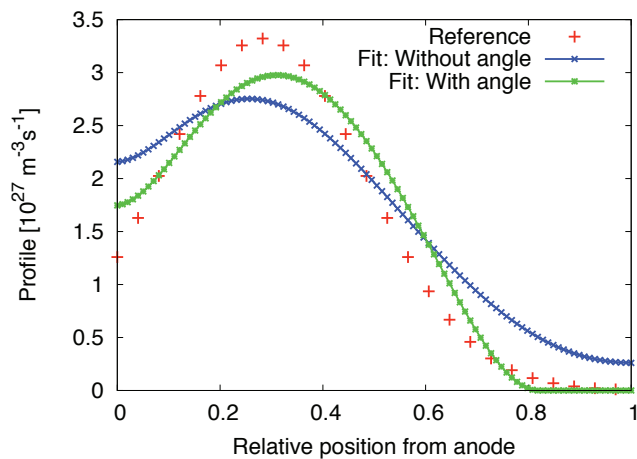
Fig. 17. Comparison between the assumed and extracted emission profiles. The emission profiles were extracted using angularly resolved emission spectra and an emission spectra measured at normal angle.
