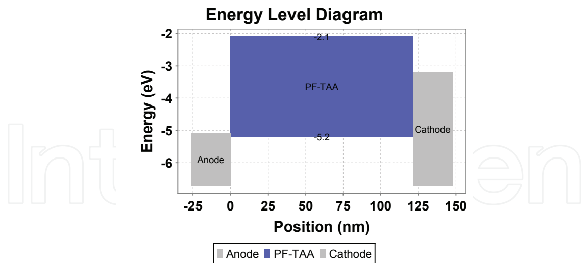
Fig. 22. Energy diagram for the simulated device. The workfunction at the anode side is held constant at 5.1 eV, while the workfunction at the cathode side \Phi_c is being optimized. The HOMO and LUMO levels are 5.2 eV, respectively 2.1 eV.
