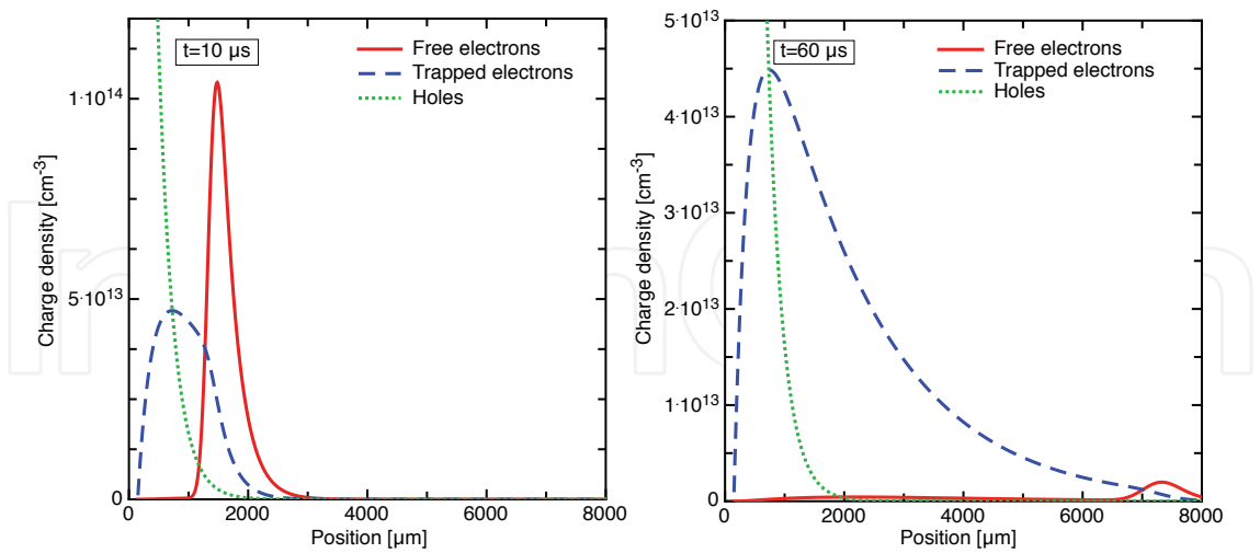
Fig. 14. Deep traps . Left: At t = 10 \mu s , the sharp packet of free electrons (red solid line) leaves the ITO electrode at position 0 \mu m and moves toward the aluminium electrode placed at position 8000 \mu m . A certain amount of charges remains trapped close to the ITO electrode (blue dashed line). Right: After 60 \mu s , those few free carriers that have not been trapped reach the aluminium electrode. Notice that trapped charges were “left behind” by the traveling free charge packet and did not move from their original position. Few trapped charges that begin to release back into the conduction band are recognizable through the slight increase of the free charges concentration around 2000 \mu m .
