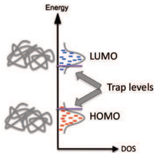
Fig. 2. Gaussian distributions of density of states and trap levels for trapped charges. As opposed to inorganic semiconductors the density of states for organic semiconductors is described by a Gaussian shape since transport is assumed to occur via a hopping process between uncorrelated sites. Thus, polymers and small molecules have broadened energy levels of their highest occupied molecular orbital (HOMO) and lowest unoccupied molecular orbital (LUMO) as shown in Fig. 2 and are described in the following way
