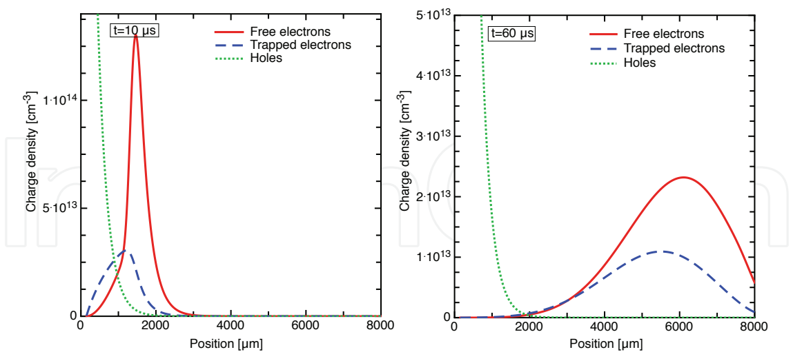
Fig. 15. Shallow traps . Left: Already at t = 10 \mu s , the free charge packet (red solid line) appears asymmetric due to the release of the weakly trapped charges (blue dashed line) around 1000 \mu m . Right: After 60 \mu s , a significant amount of free charges reaches the aluminium electrode. The fast kinetics of the trapped states makes them release back into the conduction band fast enough to follow the movement of the free electrons.
