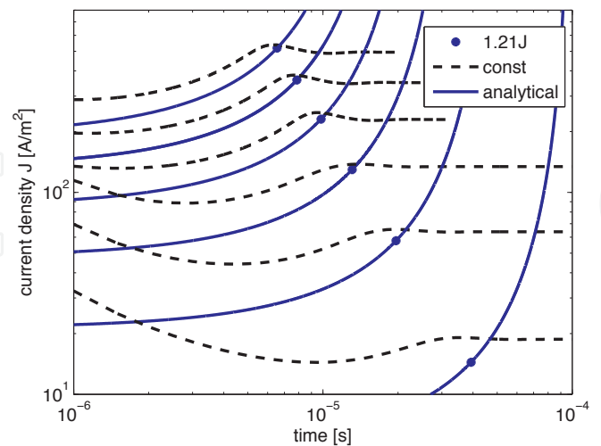
Fig. 5. Dark-injection transients for a hole-only device for a constant mobility and diffusion coefficient, the analytical solution and the generalized Einstein solution. The transients were simulated from 2 to 12 V.
