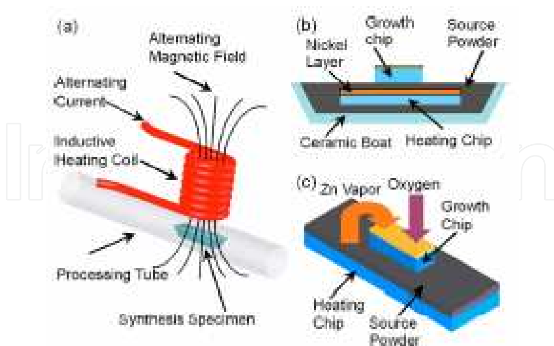
Fig. 3. Schematic illustration for ZnO nanowire synthesis setup using induction heating method (a). Cross sectional view of the synthesis specimen consisting of a heating chip, source powder, and growth chips inside a ceramic boat (b). Three-dimensional sketch of the heating chip/source powder/growth (c) [Lin et.al; Ref 11]
