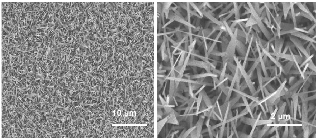
Fig. 8. ZnO nanowires grown on SiC (0001) substrates with 2 nm Au at 960 C [Wang et al; Ref 10]
