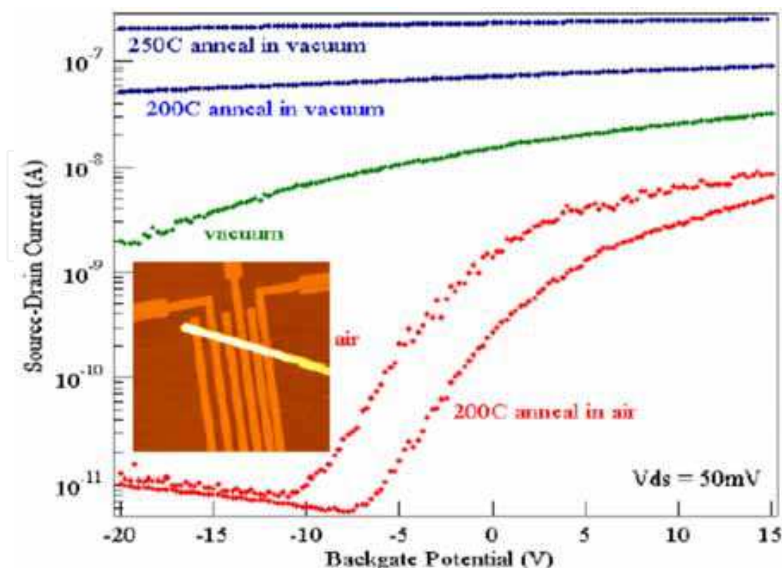
Fig. 12. ZnO nanobelt FET. Source–drain current versus gate bias for a \text{SnO}_2 FET after various treatments measured in this order: air, vacuum, 200 C vacuum anneal, 250 C vacuum anneal, 200 C air anneal. The inset shows a field effect transistor (FET) device made using a single nanobelt. [Wang et al; Ref 22]
