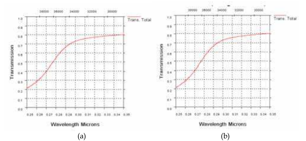
Fig. 19. UV atmospheric transmission over a horizontal path in clear maritime (23 km visibility) conditions, 1 km range (19 a). UV transmission through atmosphere over a horizontal path in desert extinction conditions, 1 km range (19b)
