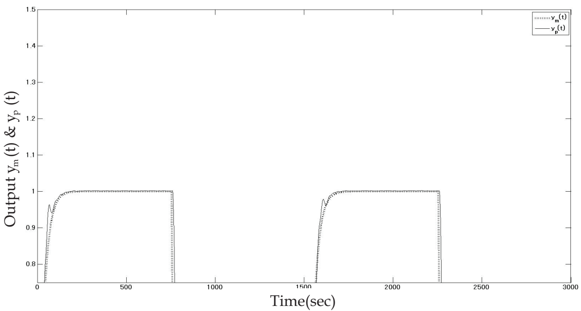
Fig. 6. Magnified upper parts of the curves in Fig. 5
