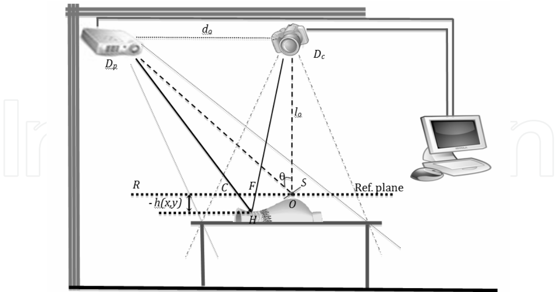
Fig. 1. Experimental setup
