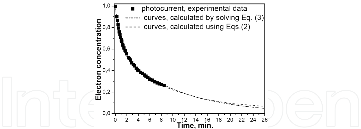
Fig. 10. Decay with time of persistent photocurrent in HPSI 4H-SiC samples at T = 300\text{ K} measured after termination of photo-excitation by interband light. After (a. Savchenko et al., 2009).
