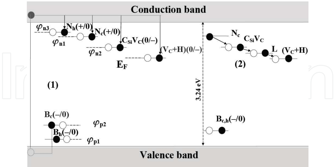
Fig. 11. Diagram of electronic transitions between impurities and defects in HPSI 4H-SiC samples stimulated by photo-excitation with interband light and after its termination. E_F is the Fermi level in the dark; \varphi_{n1} , \varphi_{n2} , \varphi_{n3} , \varphi_{p1} , and \varphi_{p2} are the Fermi quasi-levels under photo-excitation. V_{Si} energy level was not shown on diagram due to its small concentration.
