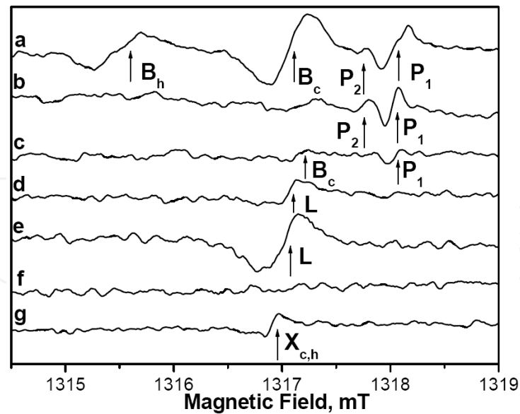
Fig. 7. Temperature-stimulated evolution of the photo-EPR spectra measured on HPSI 4H-SiC samples in the dark at 37 GHz. B_0 \perp c . The spectrum was obtained 26 h (a) after termination of photo-excitation by interband light at T = 77 K and (b-g) after a change in the temperature to (b) T = 98.5 K, (c) T = 106 K, (d) T = 86 K, (e) T = 77 K, (f) T = 140 K and (g) T = 88.5 K. After (a. Savchenko et al., 2009).
