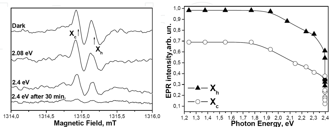
Fig. 1. Spectral dependence of the Q-band photo-EPR spectra of the X-defect measured in HPSI 4H-SiC at T = 77\text{ K} . \mathbf{B}_0 \parallel \mathbf{c} . After (b. Kalabukhova et al., 2006).
