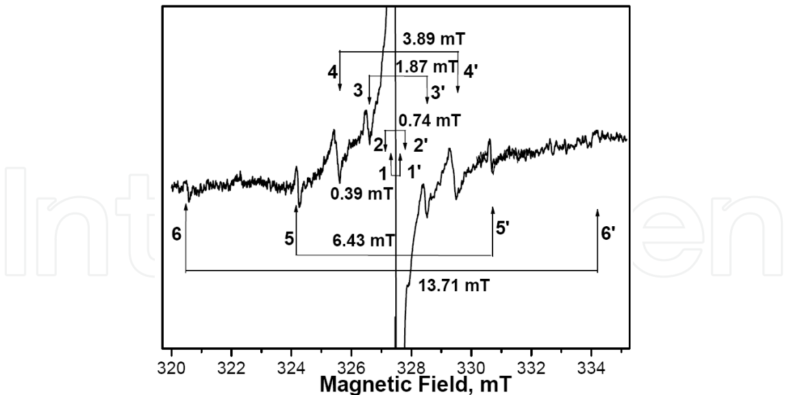
Fig. 2. X-band EPR spectrum of the X-defect measured at 77 K. B_0 \parallel c . After (b. Kalabukhova et al., 2006).
