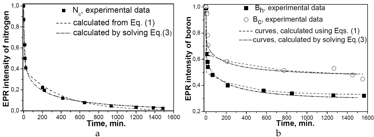
Fig. 9. Decay with time of the nitrogen (a) and boron (b) EPR signal intensity at T = 77\text{ K} measured after termination of photo-excitation of the sample by interband light. After (a. Savchenko et al., 2009).
