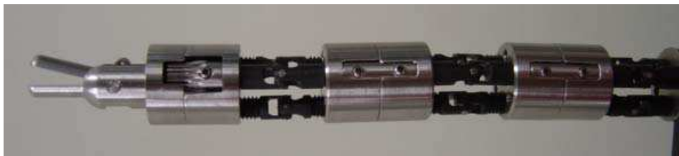
Fig. 8. Built DSD robotic forceps manipulator
