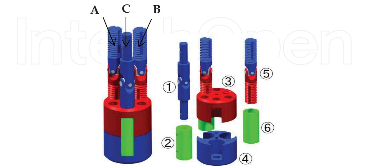
A and B: Bending linkage, C: Grasping linkage
