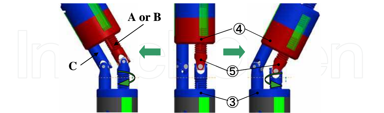
Fig. 4. Principle of bending motion
