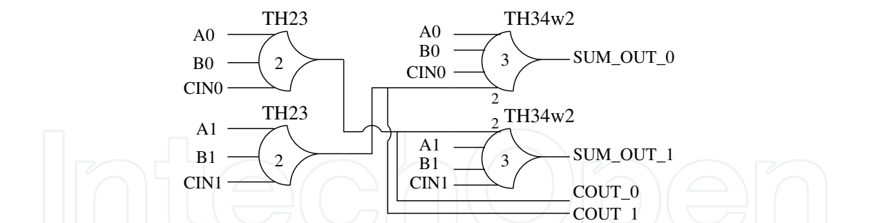
Fig. 10. Full adder NCL implementation. The circuit is splitted in two parts following the two bit coding of the NCL logic.
