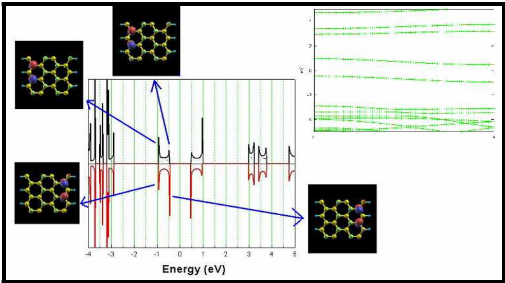
Fig. 21. Real part of the wave function, density of states and band structure for neutral nanoribbon.
