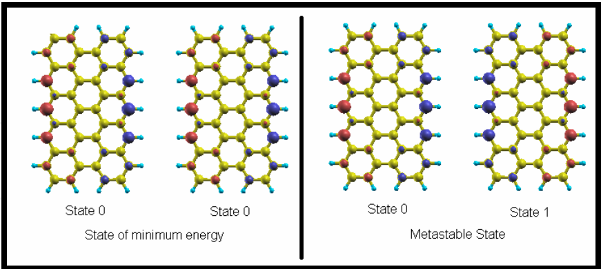
Fig. 7. Minimum energy state (left panel) and metastable state (right panel) for a system of two C 44 H 18 molecules. Red balls represent the spin up total density and blue balls represent the spin down total density.
