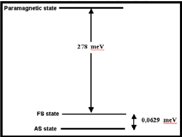
Fig. 9. Energy separation between FS state and the paramagnetic state.
