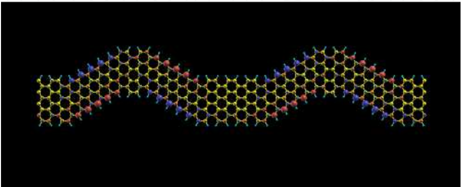
Fig. 16. Structures Z-shaped ribbons.
